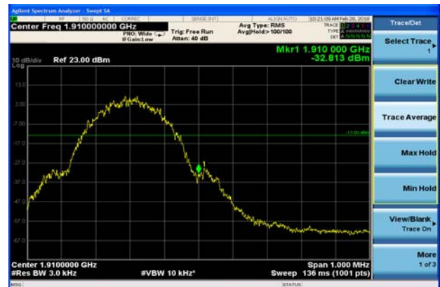
GSM 1900 GPRS CH-High
