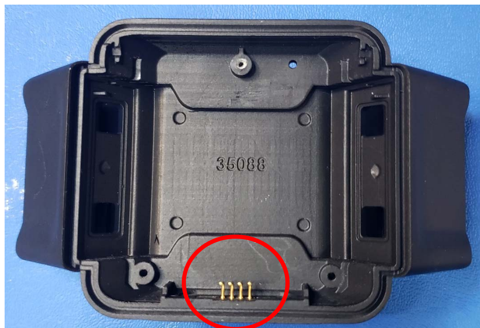
BLUtag V8 Base Enclosure showing Power Connector
