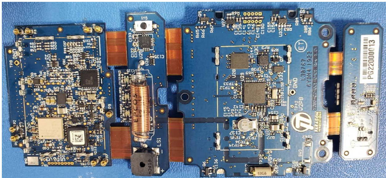
Bottom of BLUtag V8 PCB
