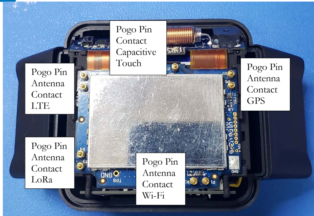
BLUtag V8 PCB Installed in Base Enclosure
