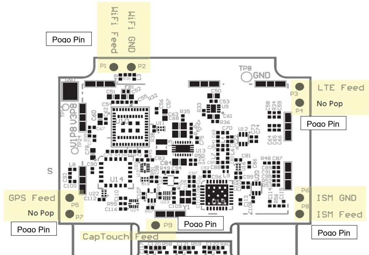
BLUtag V8 Antenna Connector Locations
