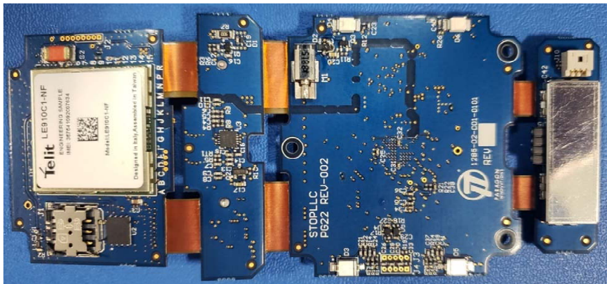
Bottom of BLUtag V8 PCB with Shields installed
