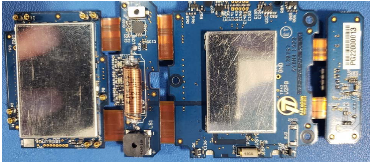
Top of BLUtag V8 PCB with Shields installed
