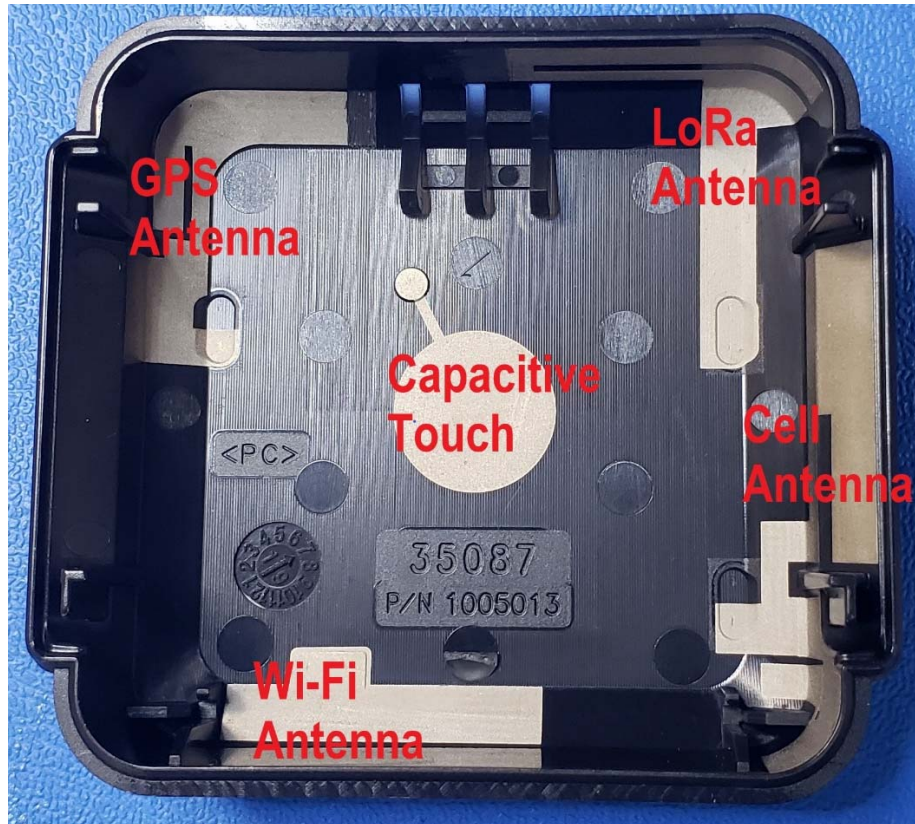
BLUtag V8 Inside Top Cover Showing Antennas
