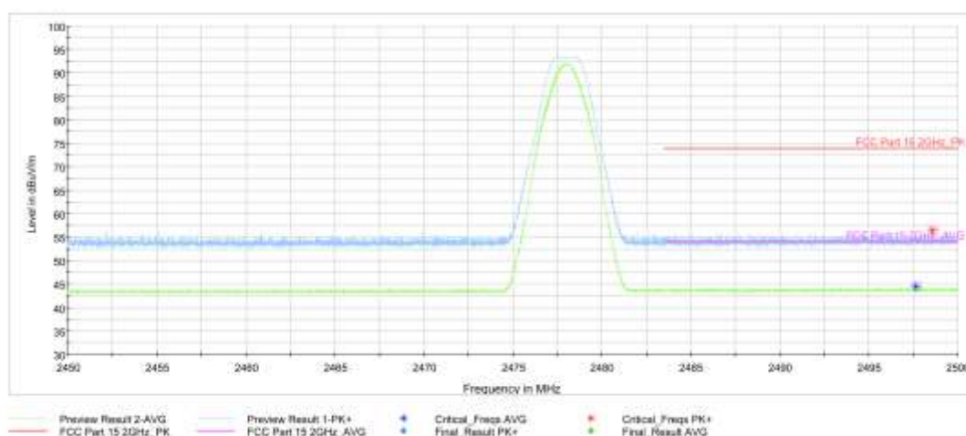
Fig.19. Frequency Band Edges: GFSK, 2478 MHz, Hopping Off, 2.45 GHz - 2.50GHz
