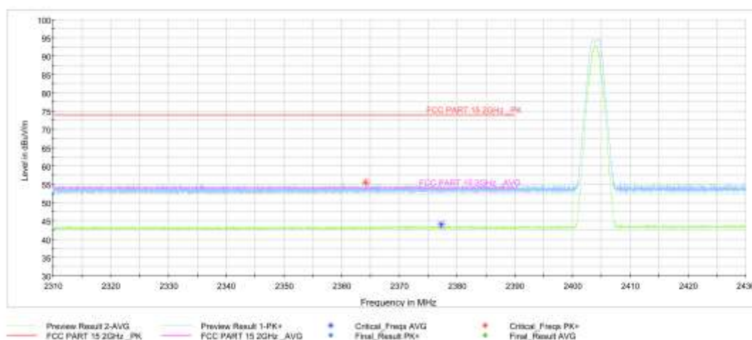
Fig.18. Frequency Band Edges: GFSK, 2404 MHz, Hopping Off, 2.31 GHz – 2.43GHz
