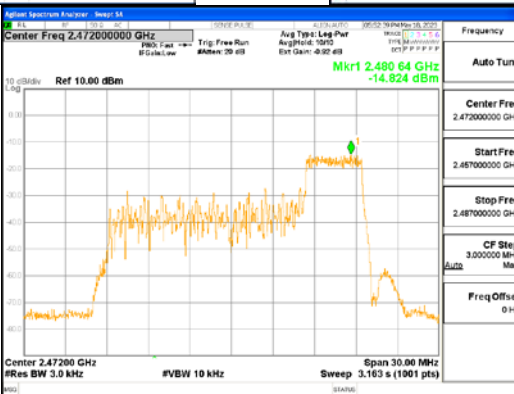
ANT L, 802.11ax_HE20_52T_High
