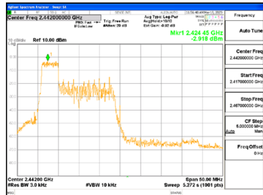
ANT L, 802.11ax_HE40_52T_Low
