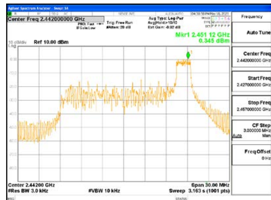
ANT L, 802.11ax_HE20_26T_High
