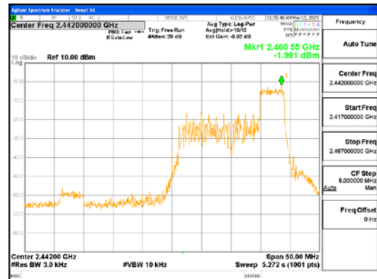
ANT L, 802.11ax_HE40_52T_High
