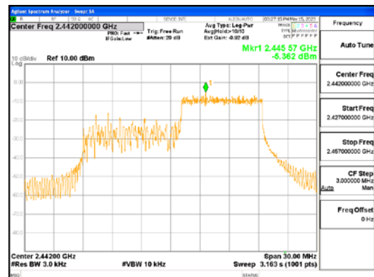
ANT L, 802.11ax_HE20_106T_High
