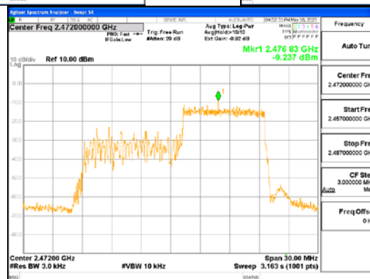
ANT R, 802.11ax_HE20_106T_High
