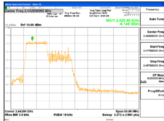
ANT L, 802.11ax_HE40_106T_Low
