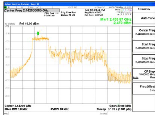
ANT L, 802.11ax_HE20_52T_Low
