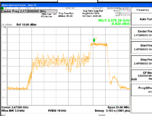
ANT R, 802.11ax_HE20_52T_High
