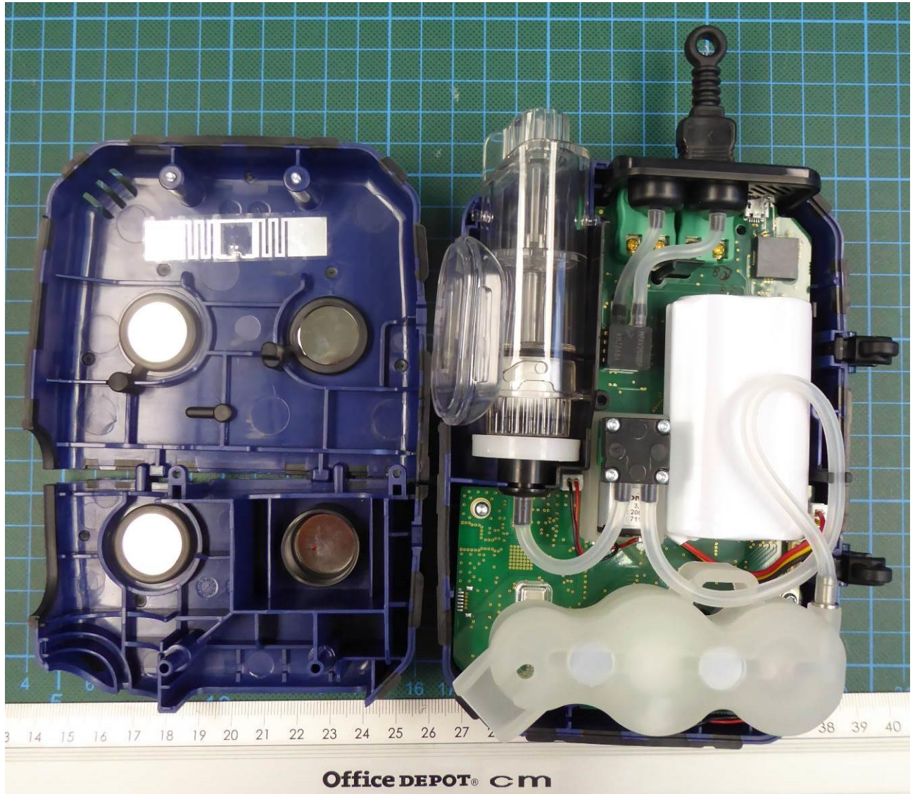
170475eut6.jpg: EUT – inside view 1
