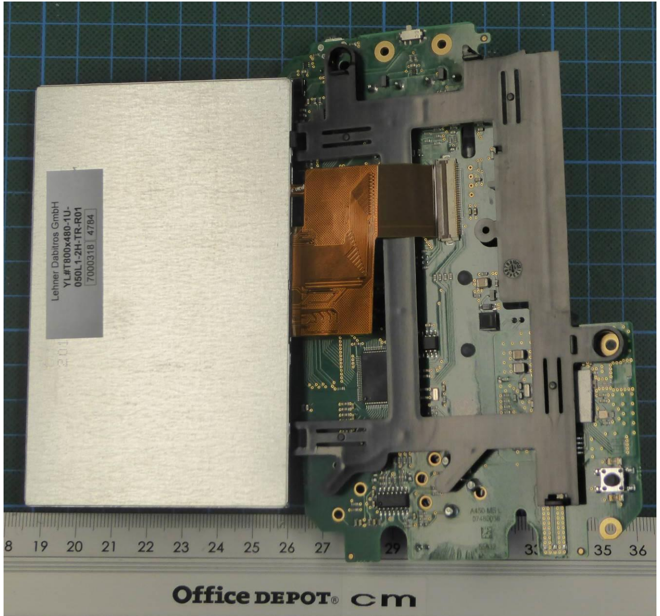
170475eut9.jpg: Main PCB with display folded away
