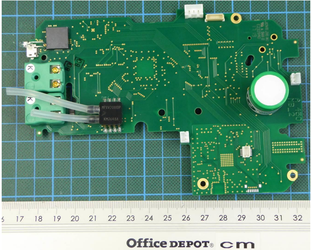
170475eut11.jpg: Main PCB – bottom view
