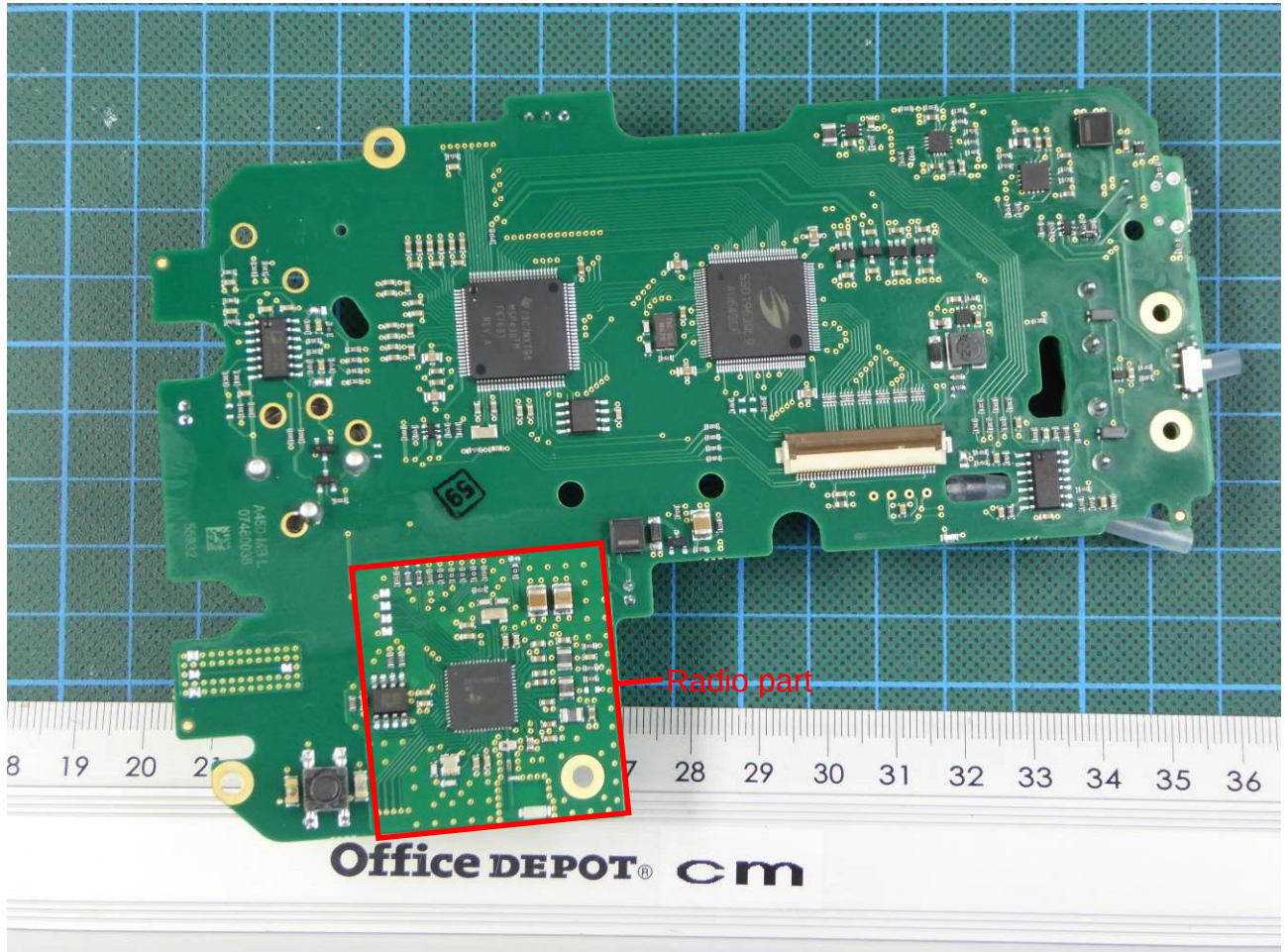
170475eut12.jpg: Main PCB – top view (without RF absorption material on RF-chip)
