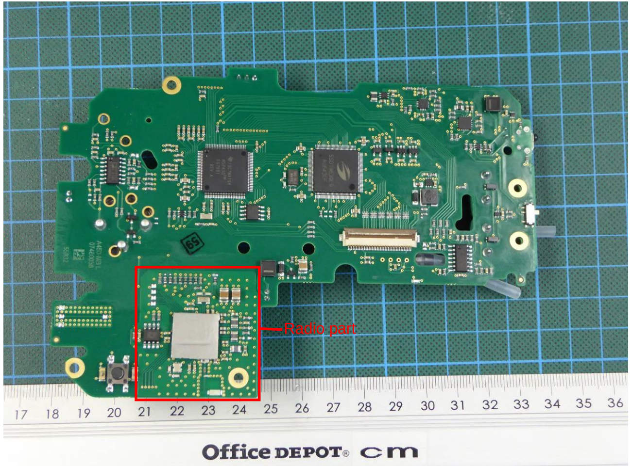
170475eut14.jpg: Main PCB – top view (with RF absorption material on RF-chip)
