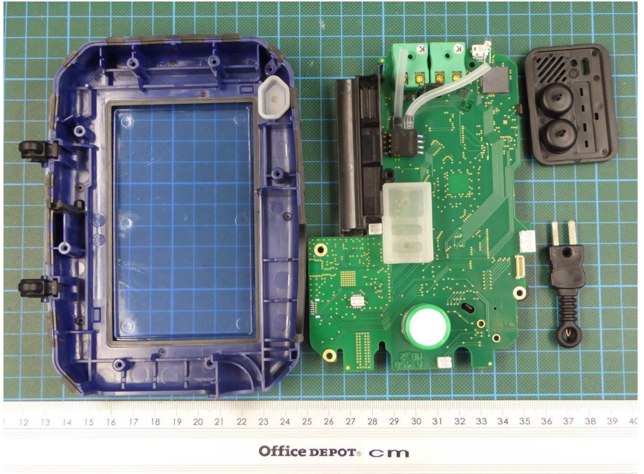
170475eut8.jpg: EUT – inside view 3
