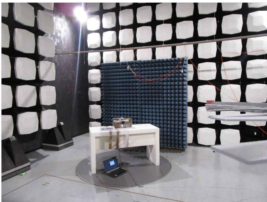
Photograph 8: EUT test setup 1 in the semi anechoic chamber, overview_EUT elevation 90°
