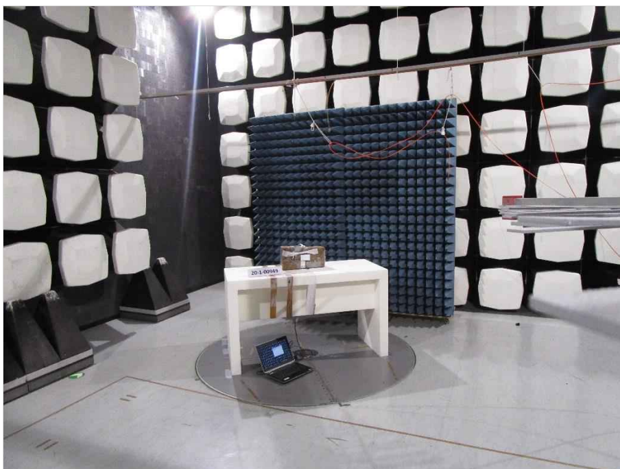
Photograph 12: EUT test setup 2 in the semi anechoic chamber, overview_EUT elevation 90°
