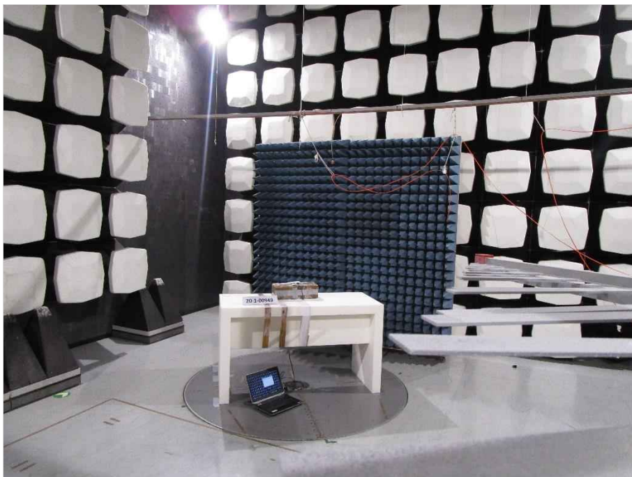
Photograph 10: EUT test setup 2 in the semi anechoic chamber, overview_EUT elevation 0°
