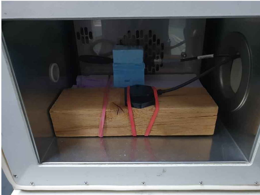
Photograph 13: EUT test setup 1 in the climatic chamber for test under extreme conditions, close up view, EUT in TX mode
