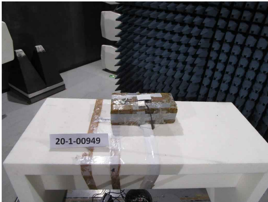
Photograph 9: EUT test setup 2 in the semi anechoic chamber, close up view_EUT elevation 0°
