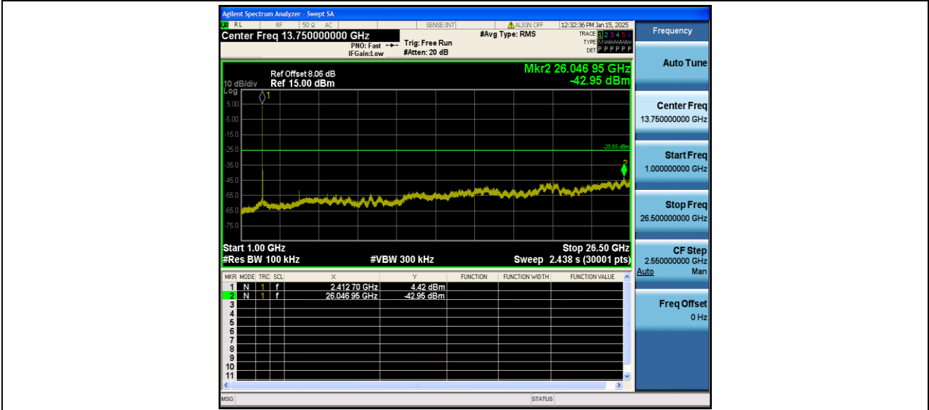
11B_Ant2_2412_0~Reference
