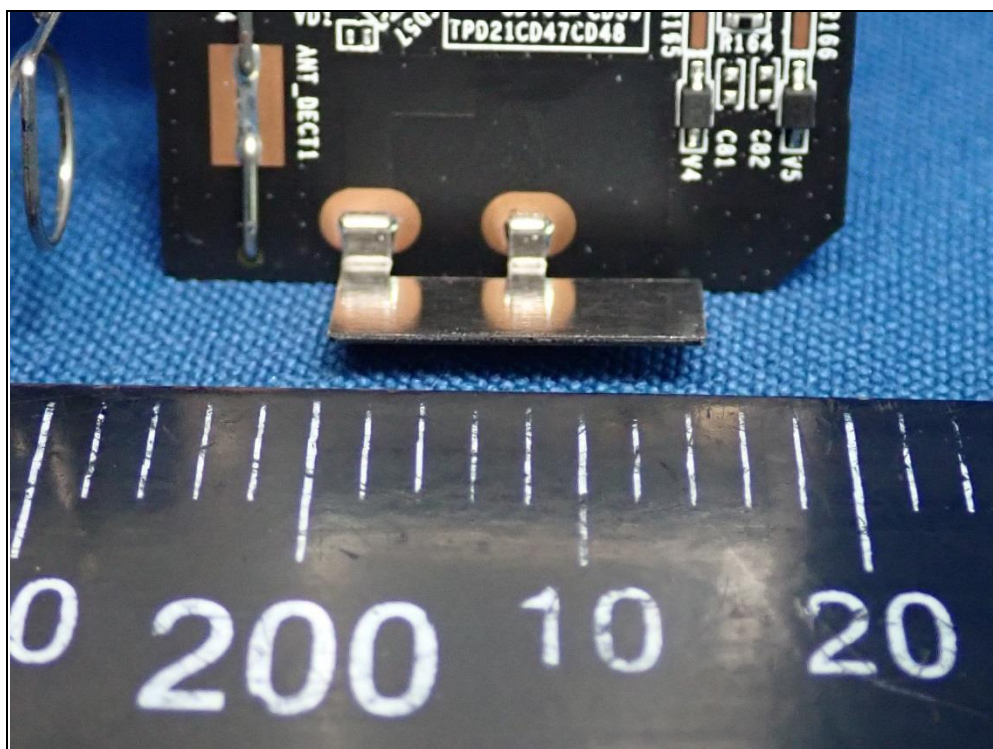
DECT antenna
