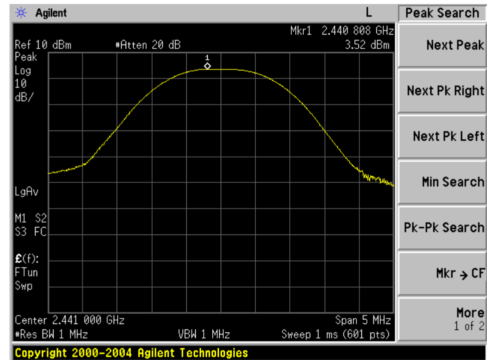
Peak output Power plot on channel 39
