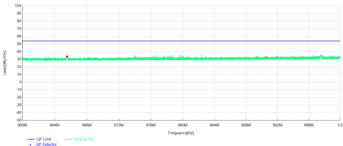
LoRa_926.9MHz: Vertical
