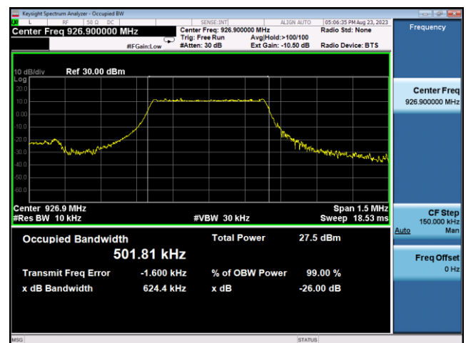
99% OBW: 926.9MHz
