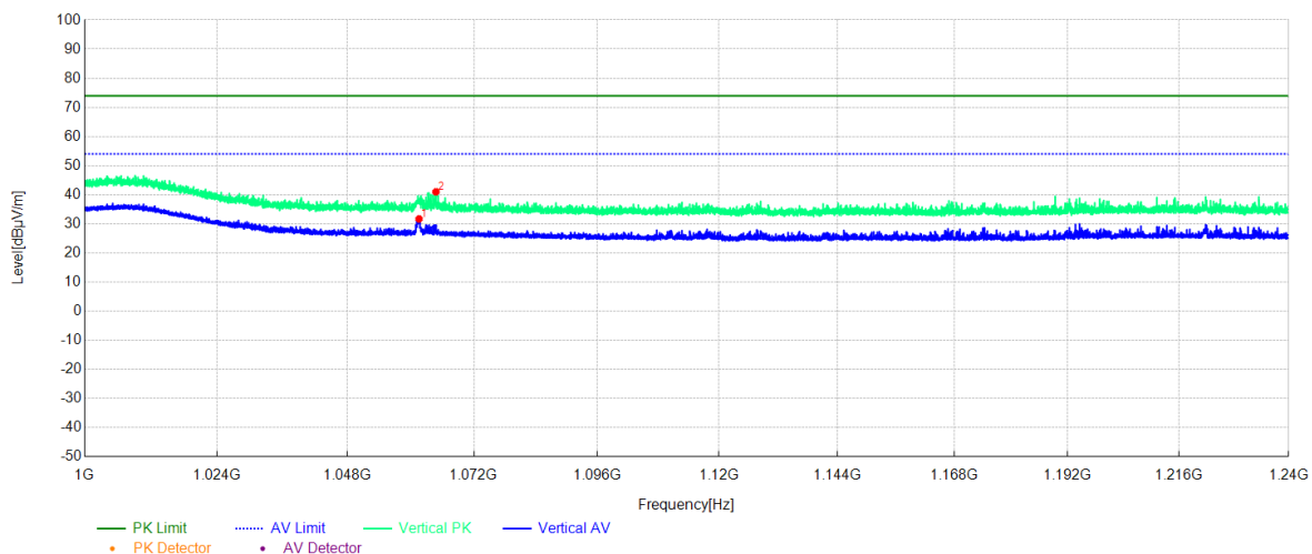
LoRa_926.9MHz: Vertical
