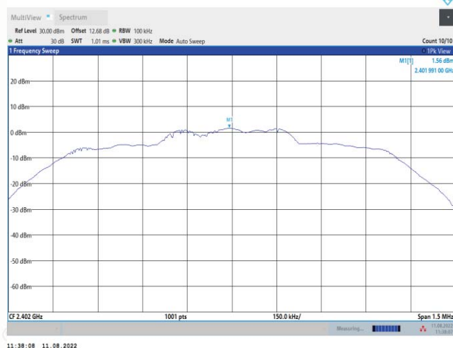
2DH5_Ant1_2402_30~1000
