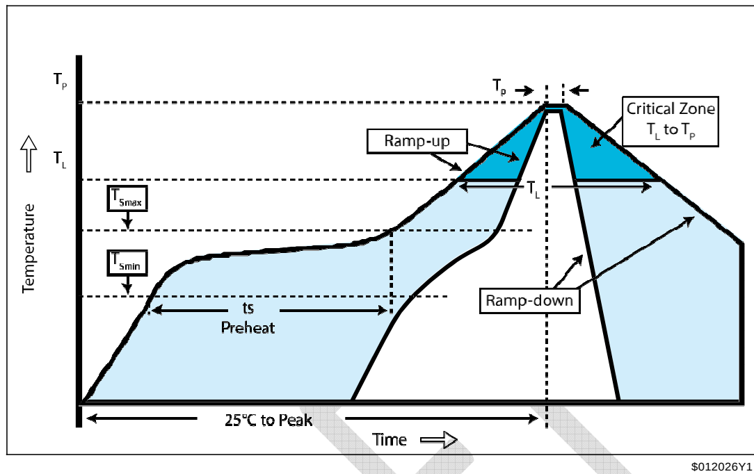
Figure 4. Soldering profile
