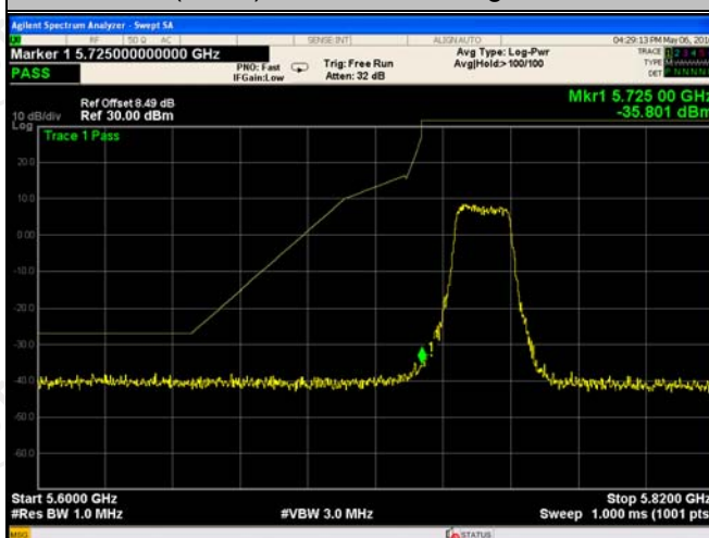
11ac(HT40) band IV Band edge-left side
