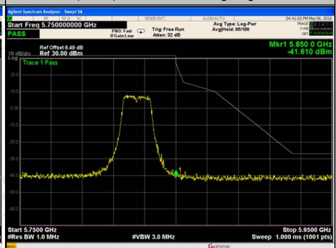
11ac(HT40) band IV Band edge-right side
