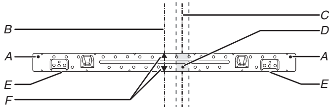
No Wall Studs at End Holes Figure 2
