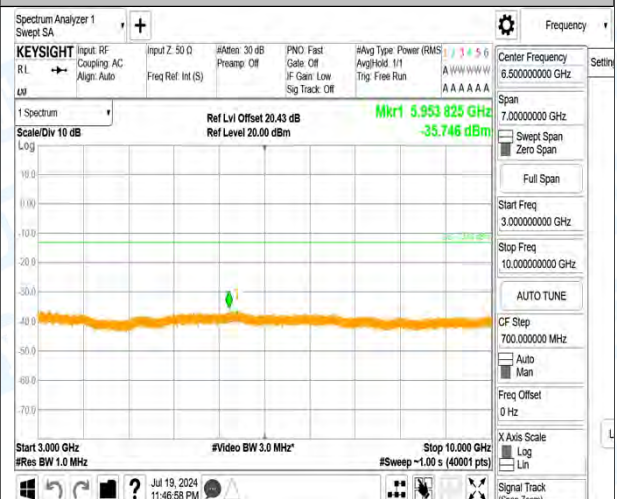
Band5_10MHz_16QAM_20600_1RB#0_3000~10000_3000~10000
