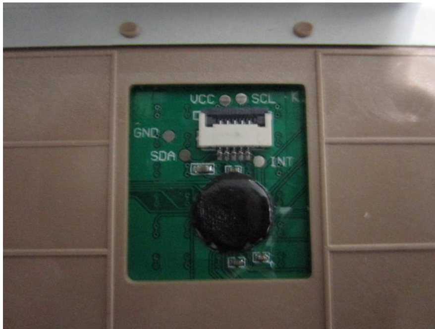
EUT- PCB 4 View
