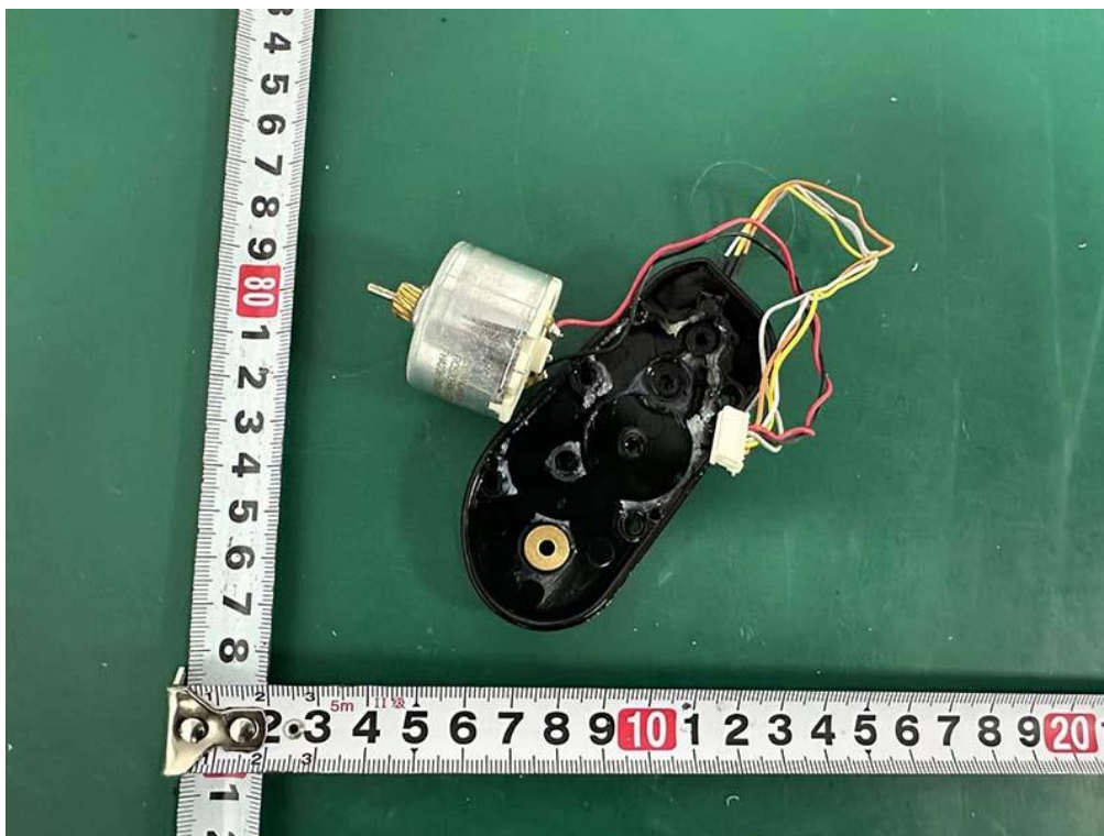
Internal photos M/N: SDL70
