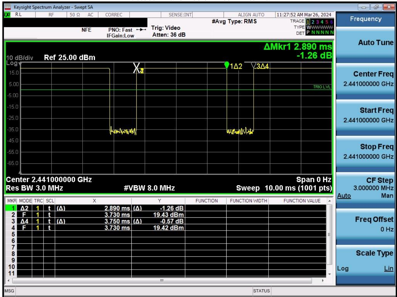
Equation 7-2 Bluetooth Antenna 1 Duty Cycle Calculation
