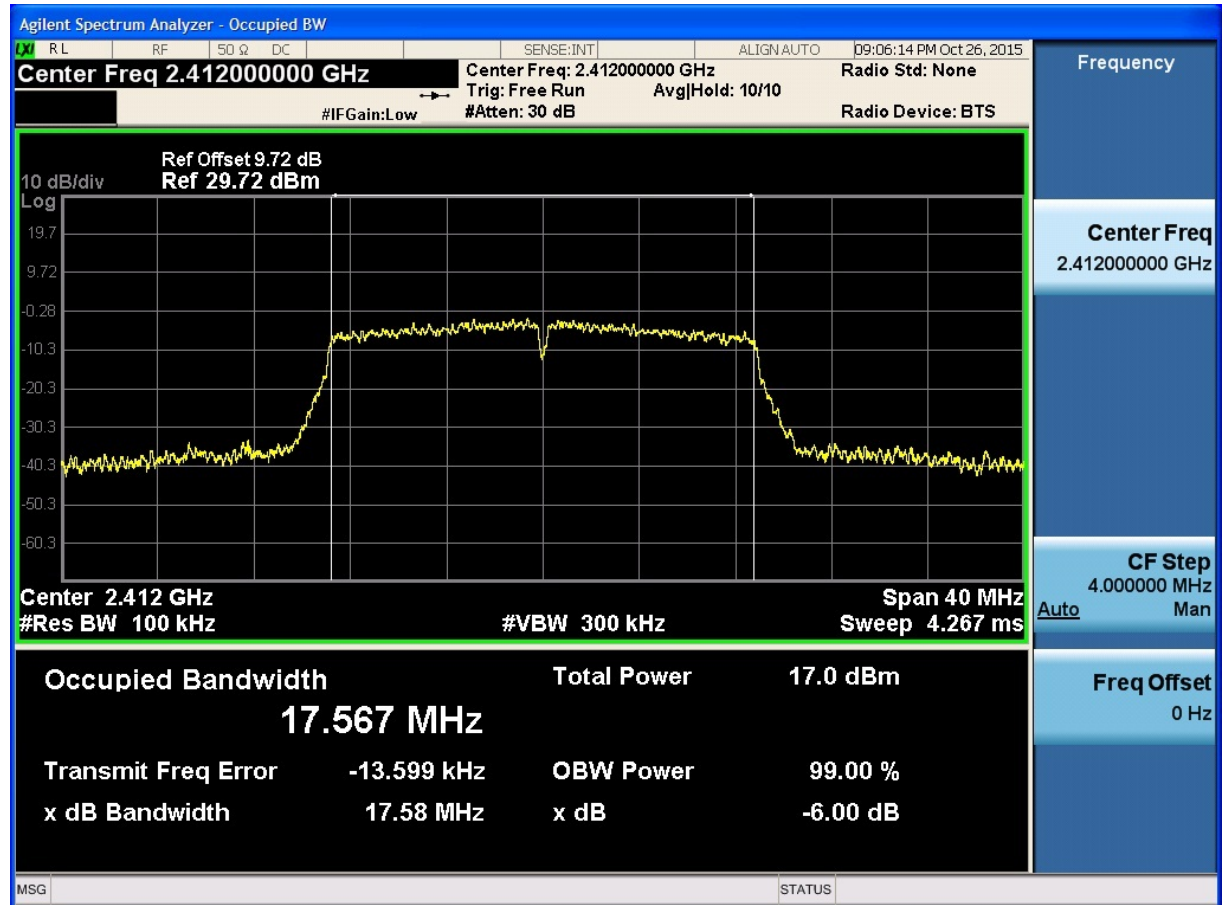
(Plot 4.7.3 A: Channel 1: 2412MHz @ 802.11n HT20)
