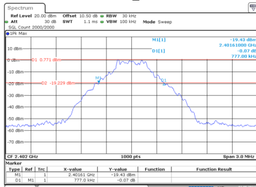
GFSK_Low
