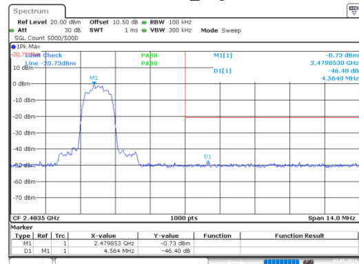
8DPSK_High
