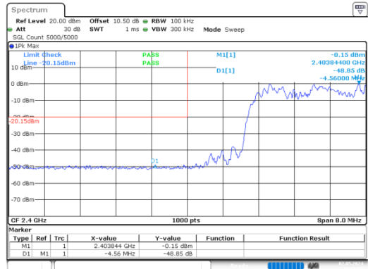
8DPSK_Hopping_Lower
