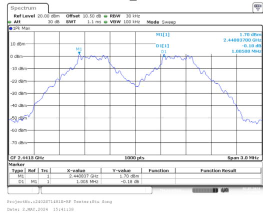
GFSK_Middle
