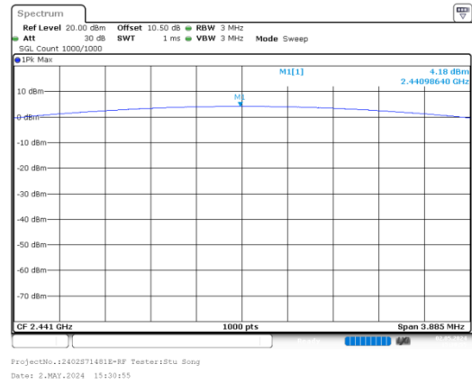
GFSK_Middle
