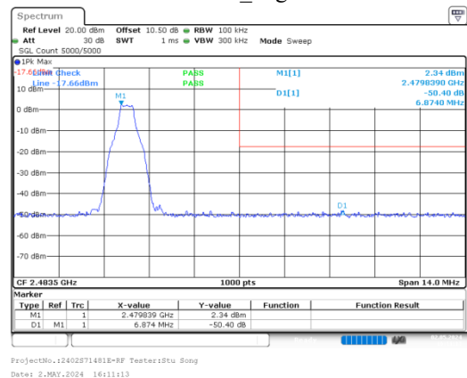
GFSK_High
