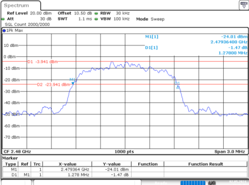
8DPSK_High
