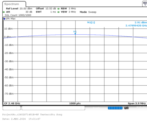
GFSK_High
