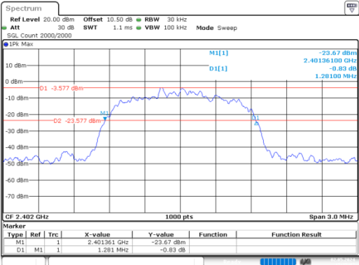
8DPSK_Low
