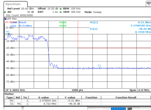
8DPSK_Hopping_Upper
