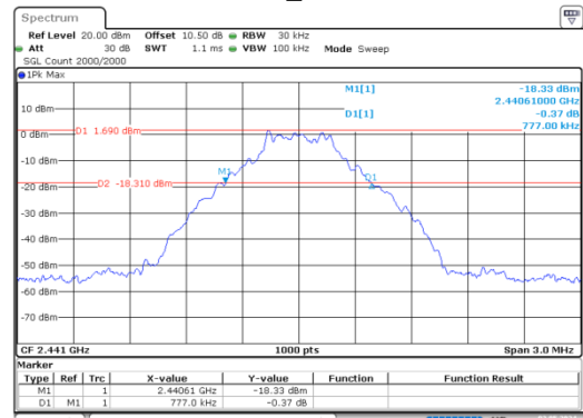
GFSK_Middle
