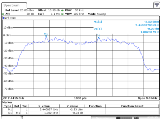
8DPSK_Middle
