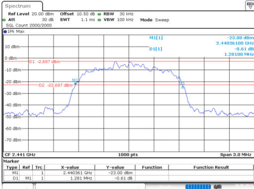
8DPSK_Middle
