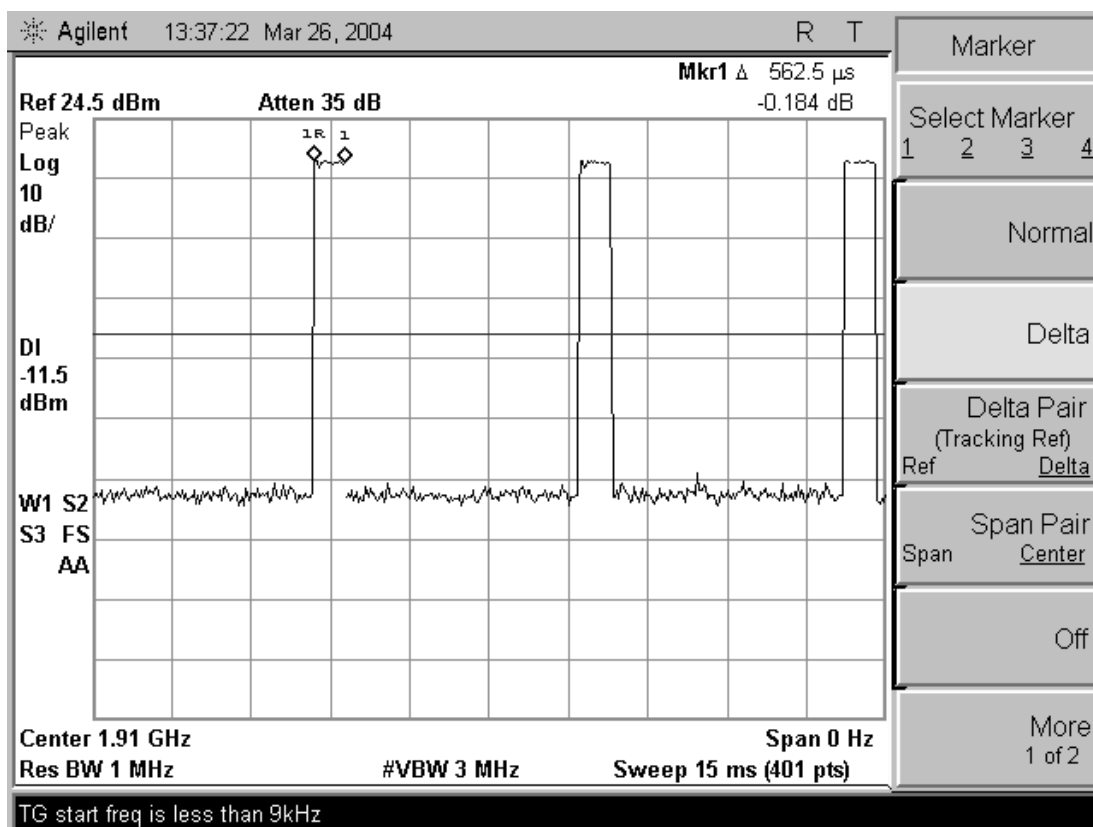
figure 2 (Modulation Characteristics)
