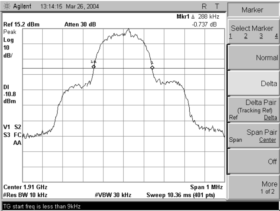
figure 5 26dB Bandwidth f_c = 1909.55 \text{ MHz}
