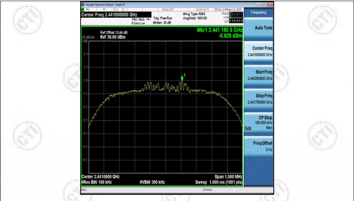
2DH5-Ant1-2441-0~Reference-PASS
