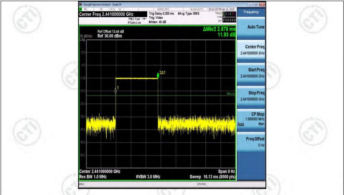
DH5-Ant1-Hop-PASS
