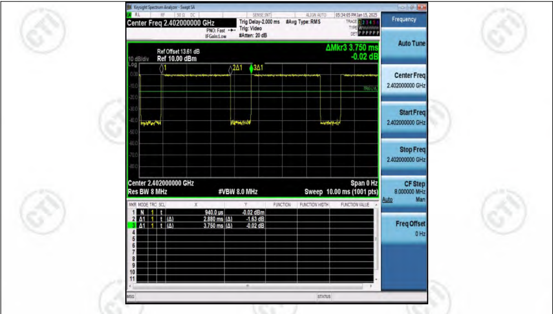
NTNV-3DH5-Ant1-2402
