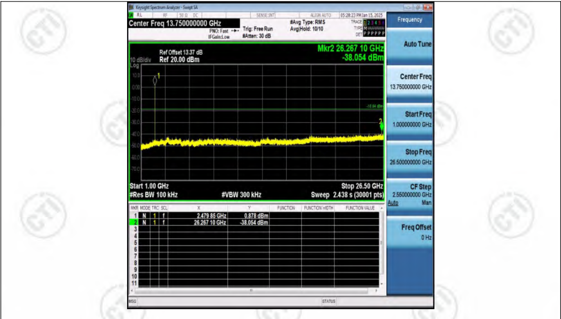
DH5-Ant1-2480-1000~26500-PASS
