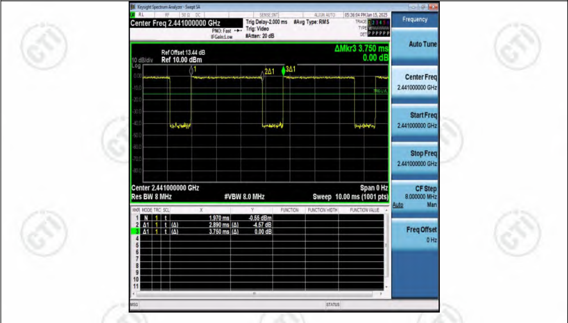
NTNV-3DH5-Ant1-2441
