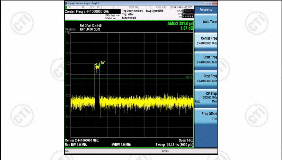
2DH1-Ant1-Hop-PASS
