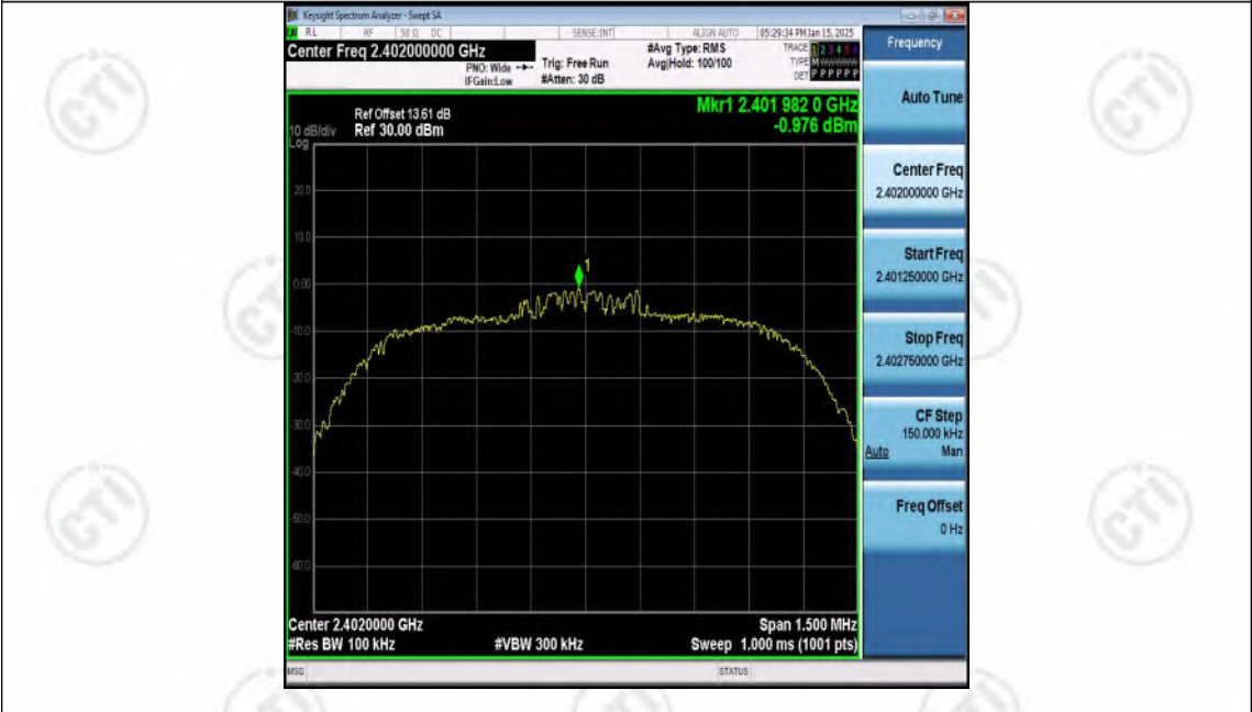
2DH5-Ant1-2402-0~Reference-PASS
