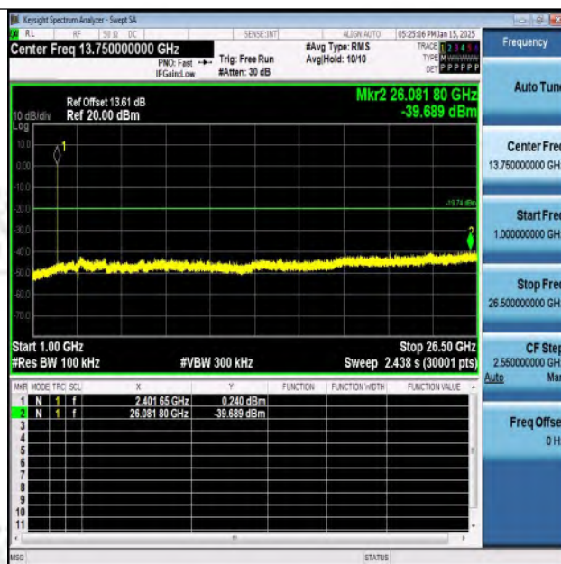
DH5-Ant1-2402-1000~26500-PASS
