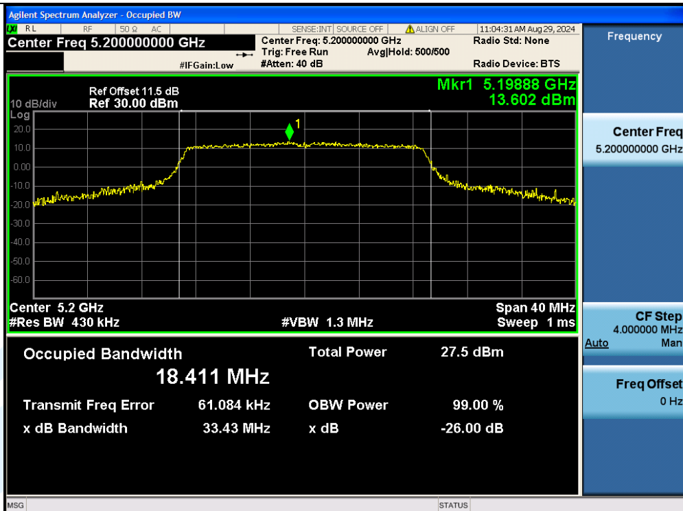
11AC20MIMO-Ant3-5200
