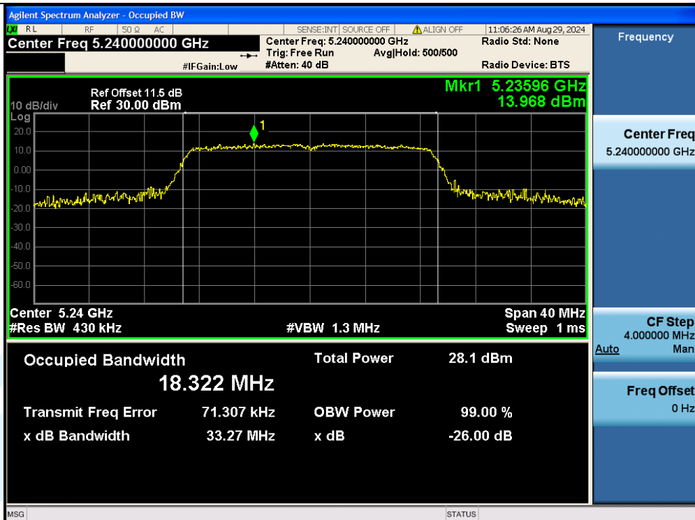
11AC20MIMO-Ant3-5240
