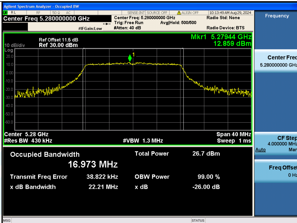
11A-Ant3-5280
