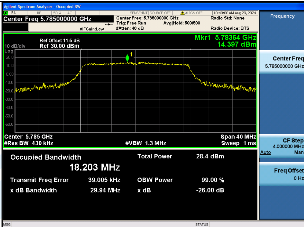
11N20MIMO-Ant3-5785
