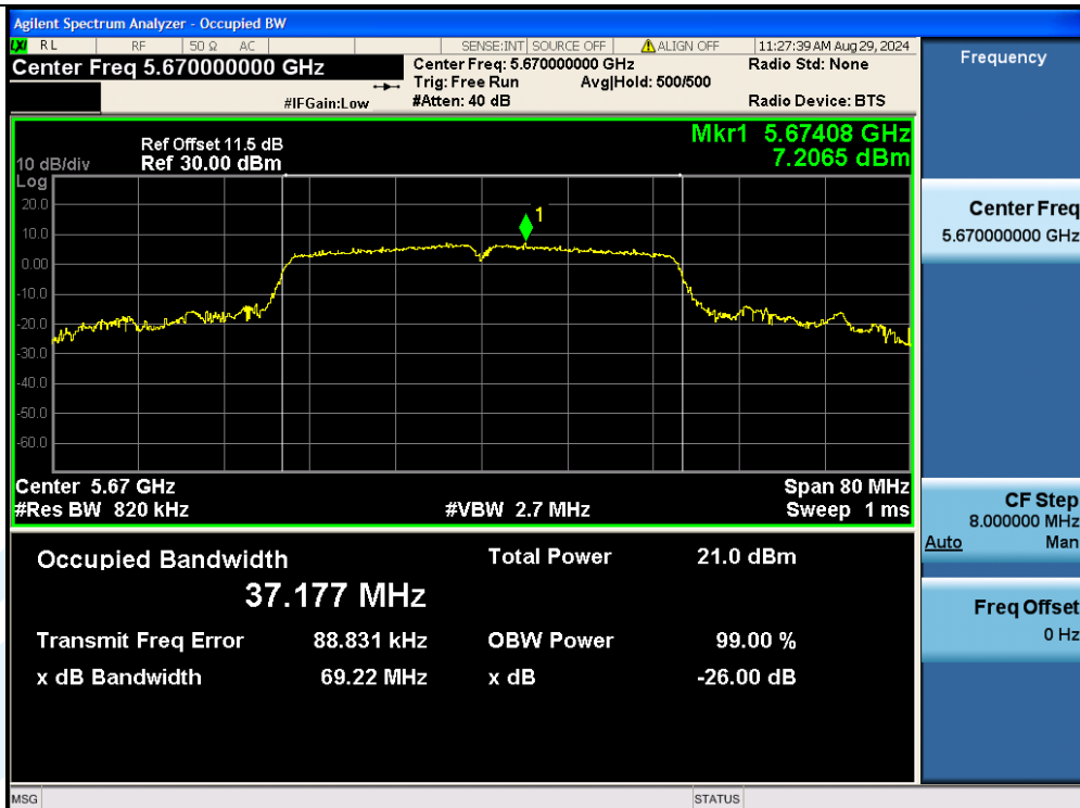
11AC40MIMO-Ant3-5670
