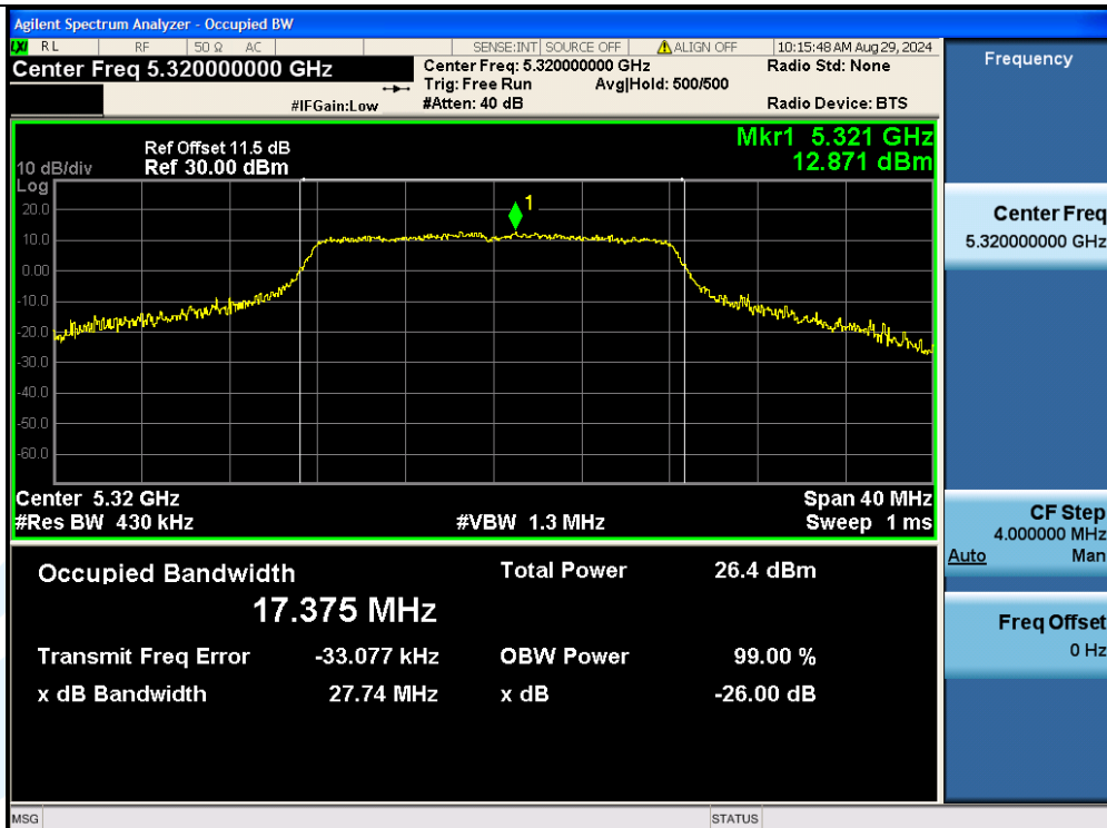
11A-Ant3-5320
