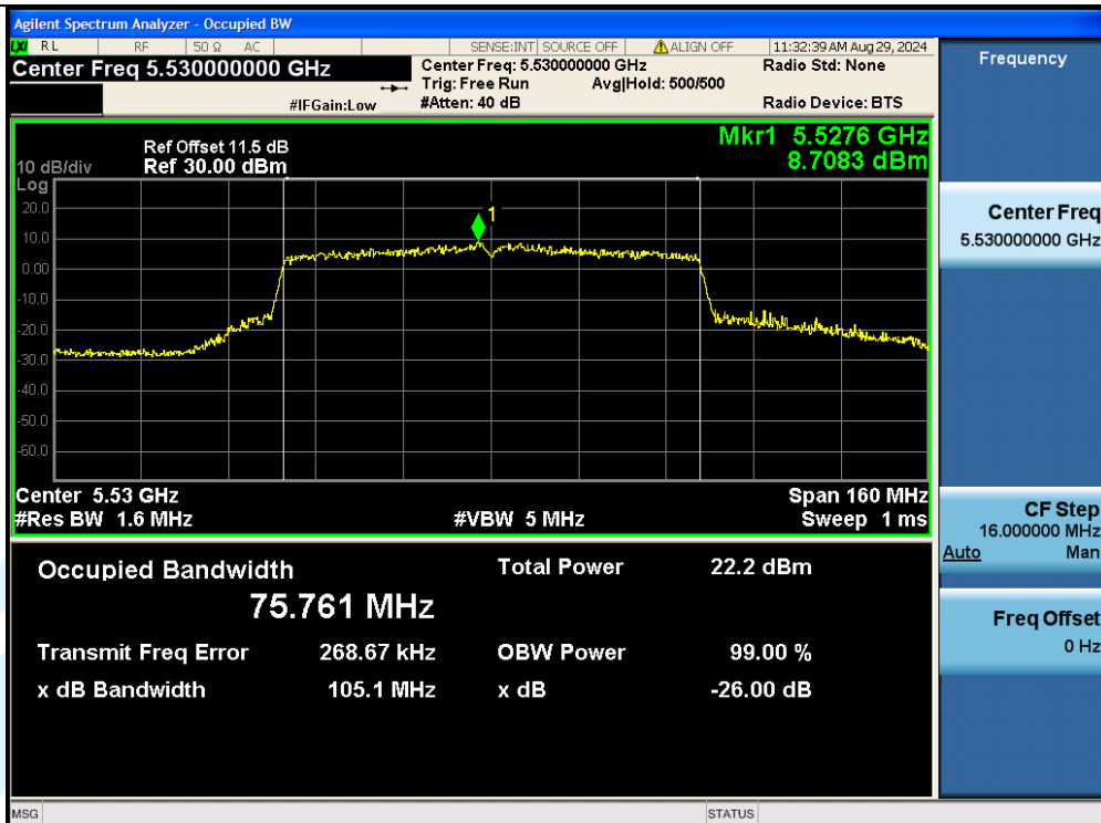
11AC80MIMO-Ant3-5530
