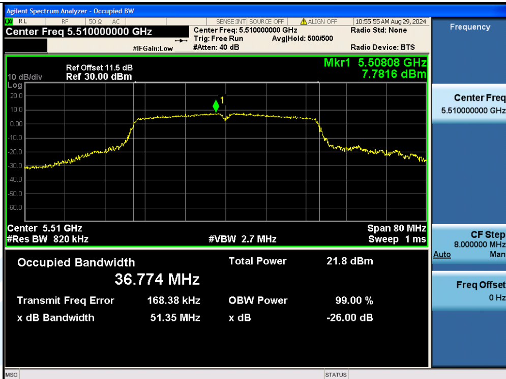
11N40MIMO-Ant3-5510
