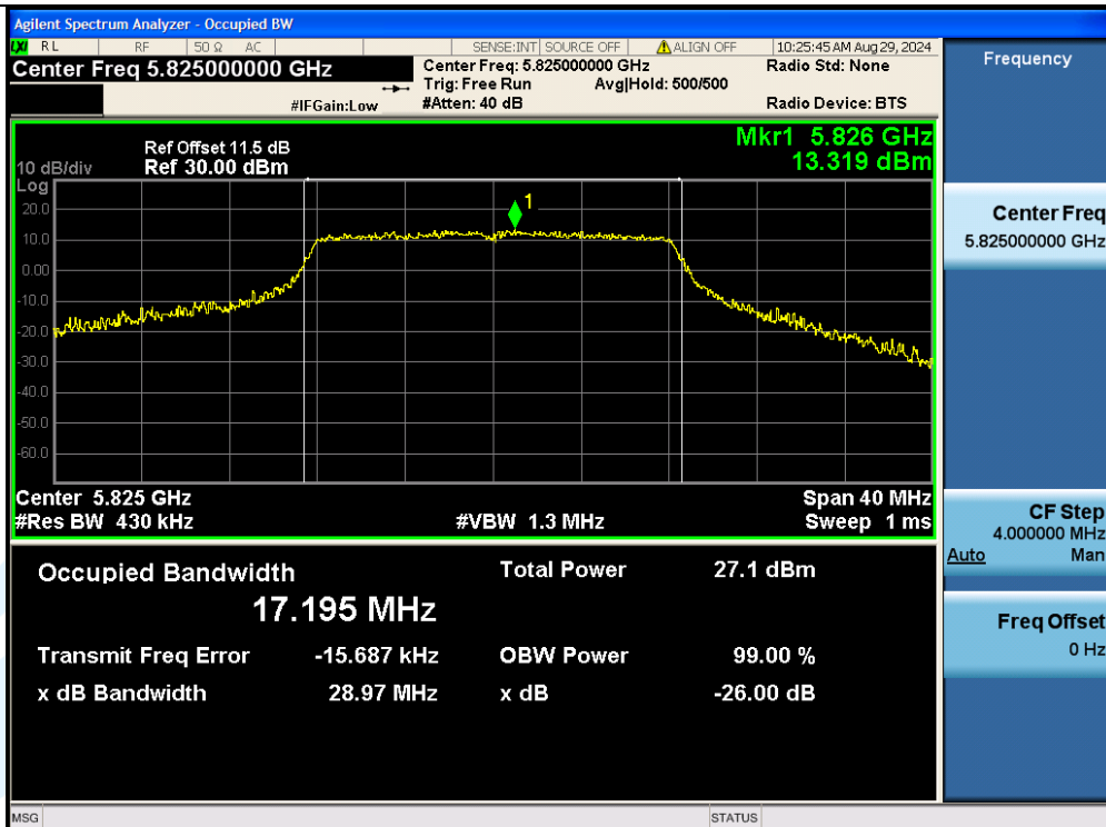
11A-Ant3-5825
