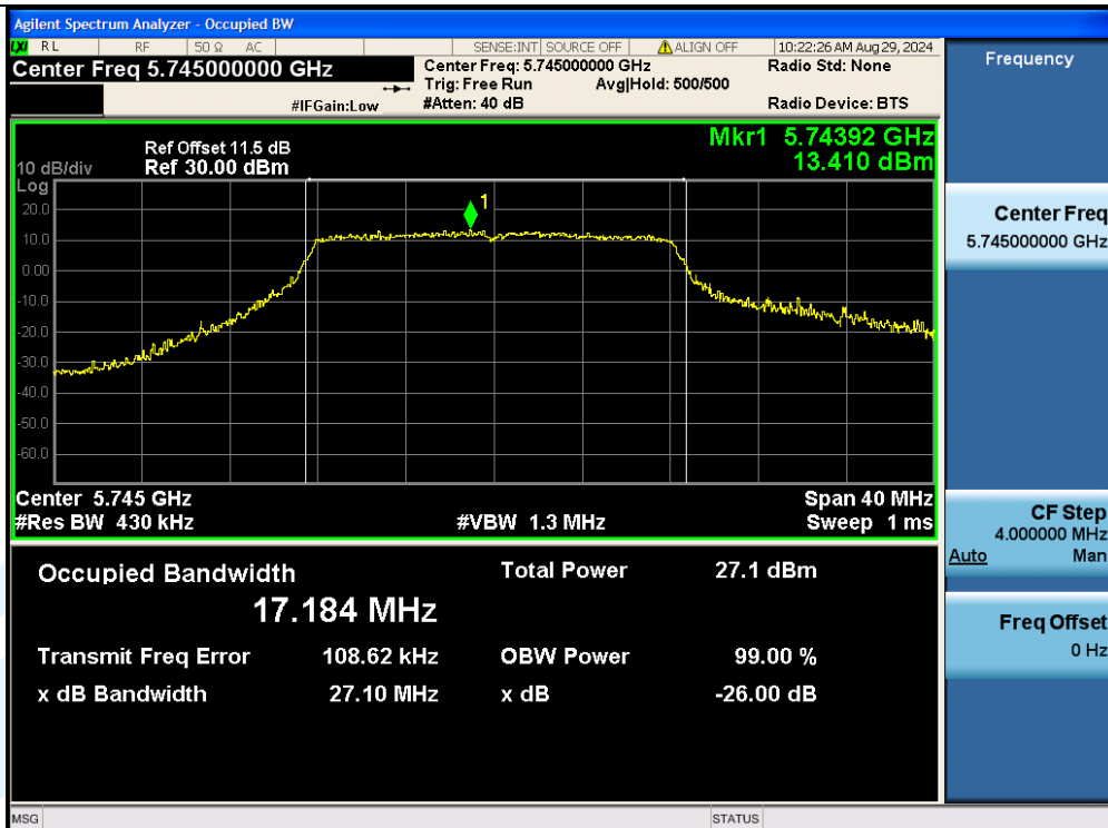
11A-Ant3-5745
