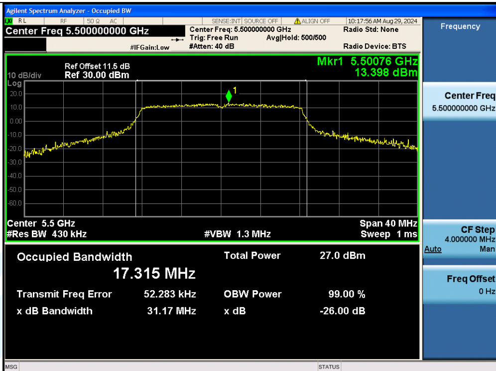
11A-Ant3-5500
