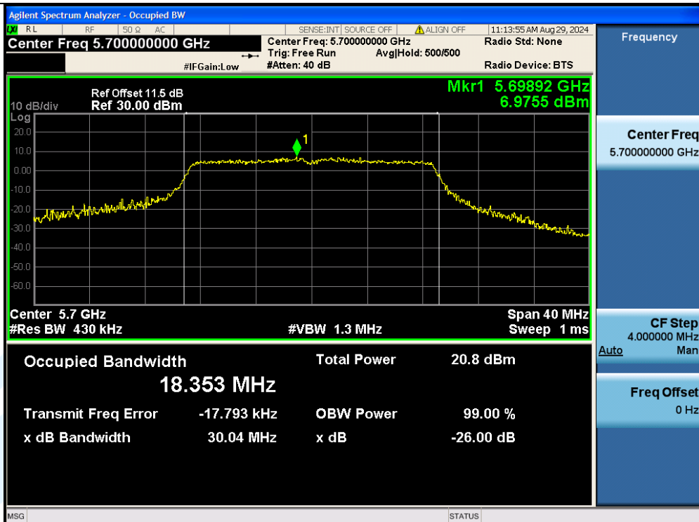
11AC20MIMO-Ant3-5700
