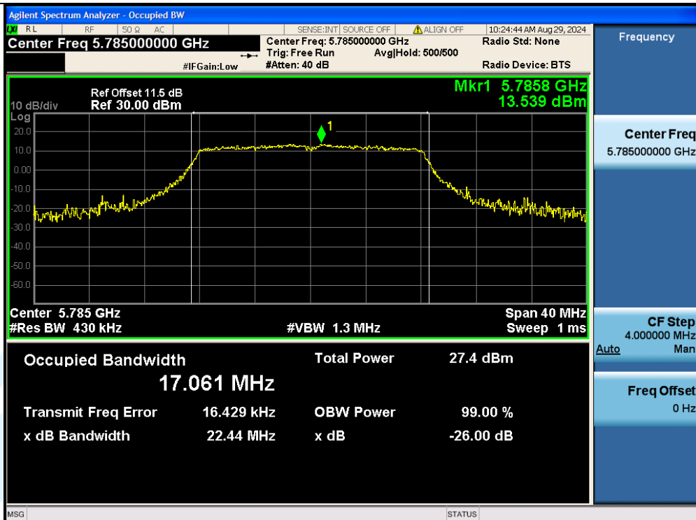
11A-Ant3-5785
