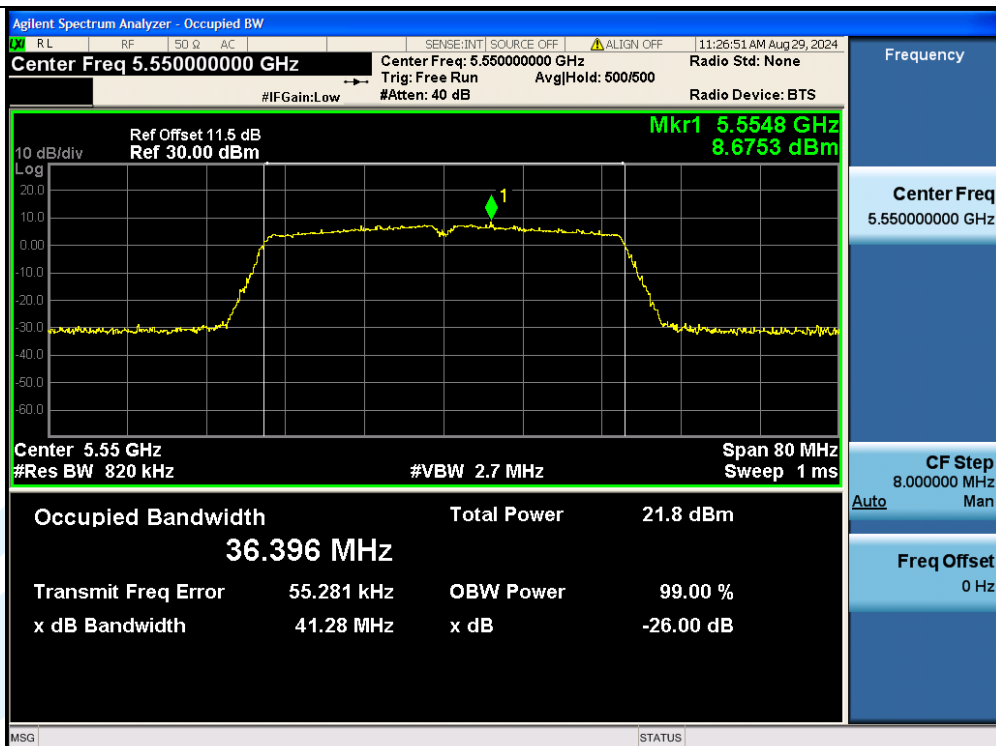
11AC40MIMO-Ant3-5550
