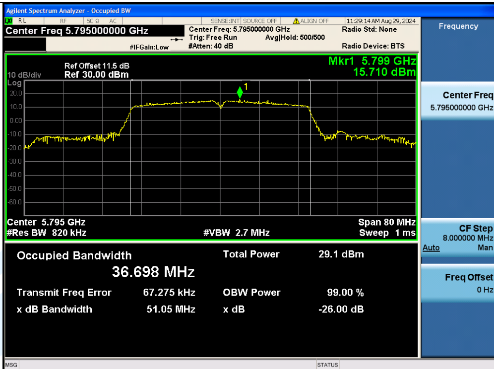
11AC40MIMO-Ant3-5795
