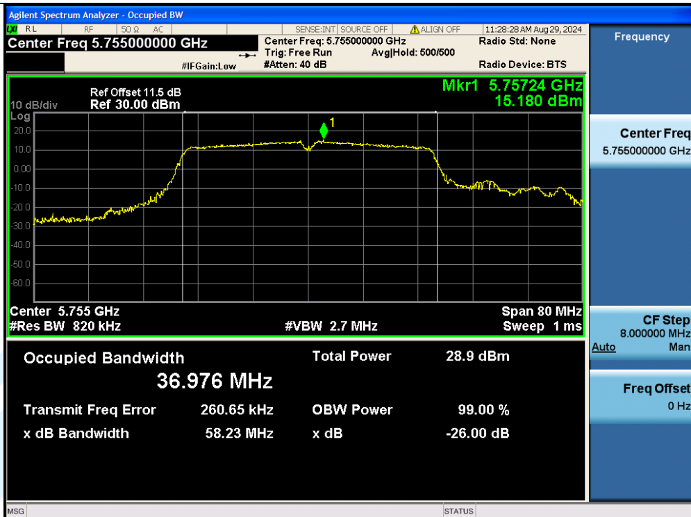
11AC40MIMO-Ant3-5755
