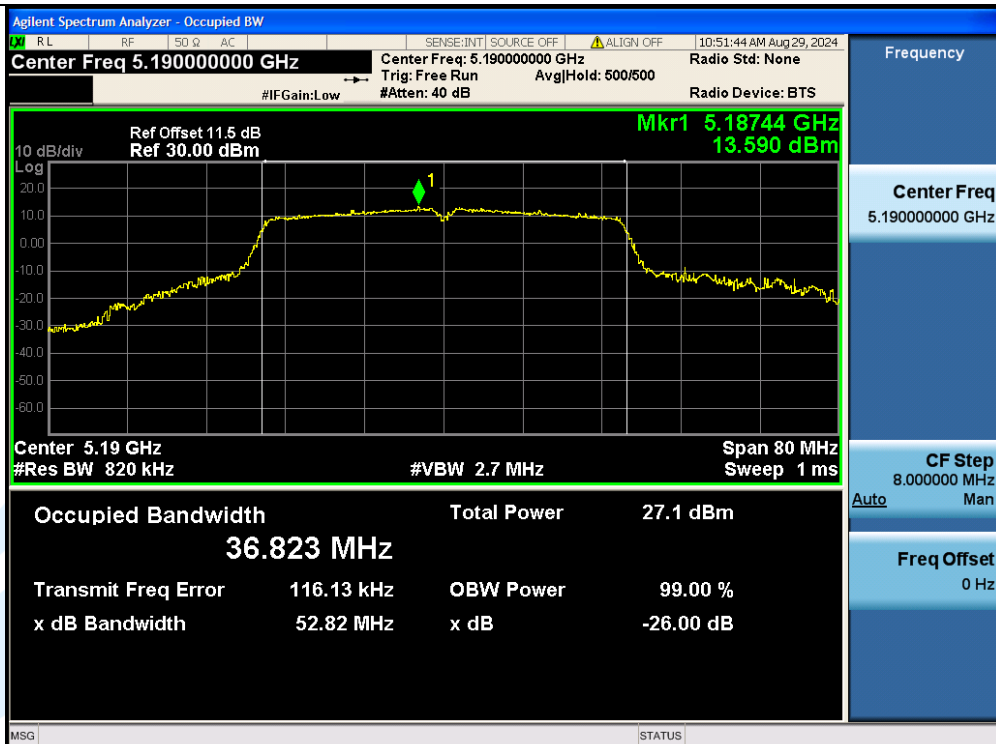
11N40MIMO-Ant3-5190
