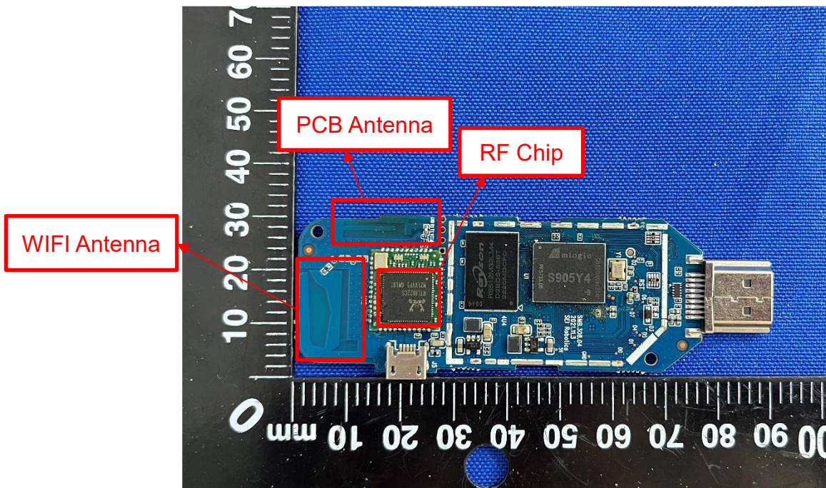
MAIN BOARD REAR VIEW (WITHOUT SHIELDING)
