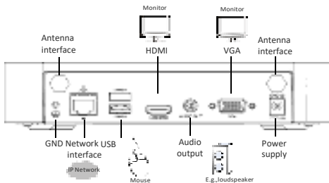
Figure 4-1 NVR Interfaces
