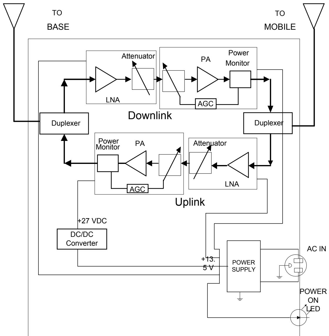
CBDA-10W80 ELECTRICAL SCHEMATICS
