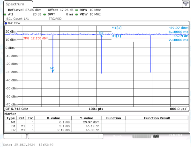
NTNV-11A-CDD-Ant2-5745
