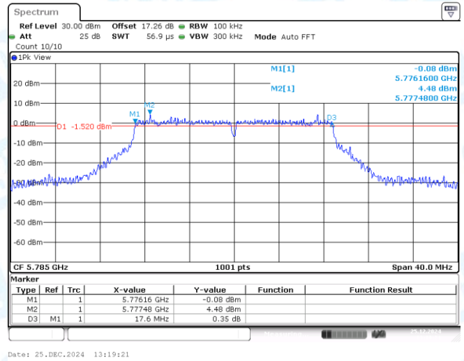
11N20MIMO-Ant2-5785-PASS
