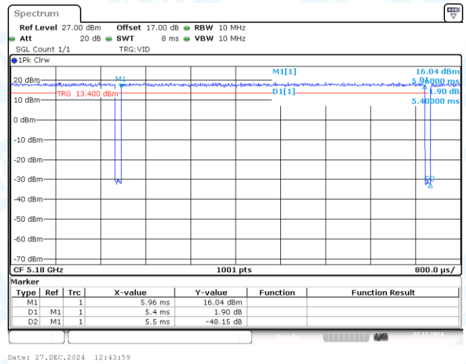
NTNV-11AC20MIMO-Ant2-5180
