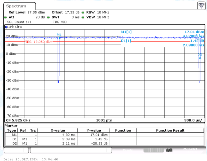
NTNV-11A-CDD-Ant2-5825
