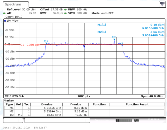
11AX20MIMO-Ant2-5825-PASS
