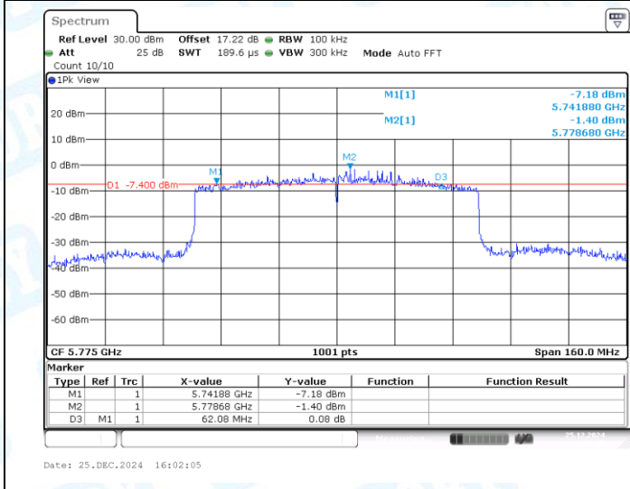
11AX80MIMO-Ant1-5775-PASS
