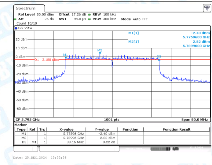
11AX40MIMO-Ant2-5795-PASS
