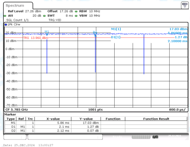
NTNV-11A-CDD-Ant2-5785
