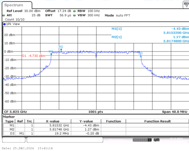
11AX20MIMO-Ant1-5825-PASS
