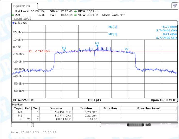
11AX80MIMO-Ant2-5775-PASS
