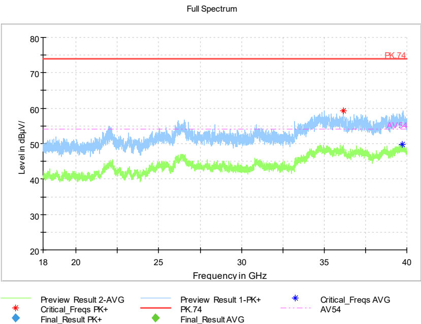
Frequency Range: 18GHz -40GHz Detector: Av mode and PK mode Test Mode: 802.11ac(VHT40)
