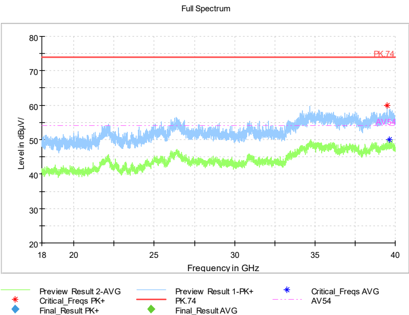
Frequency Range: 18GHz -40GHz Detector: Av mode and PK mode Modulation type: 802.11a
