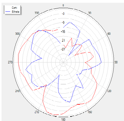
H Theta=90 freq=5800MHz
