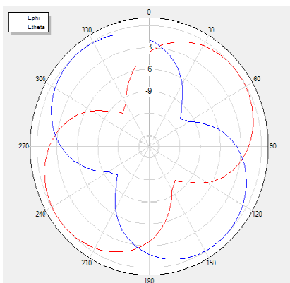
H Theta=0 freq=5800MHz
