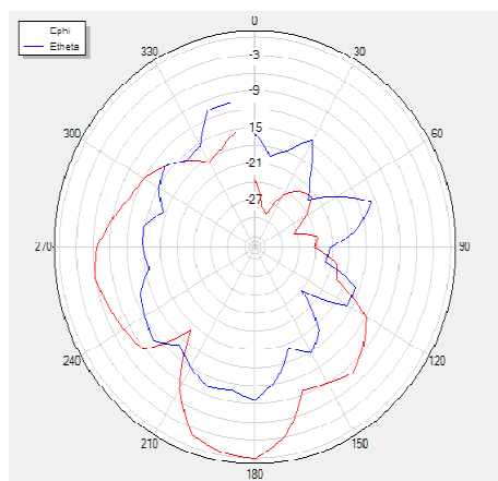
H Theta=90 freq=5400MHz
