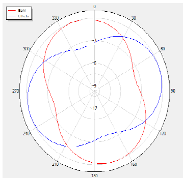
H Theta=0 freq=2450MHz
