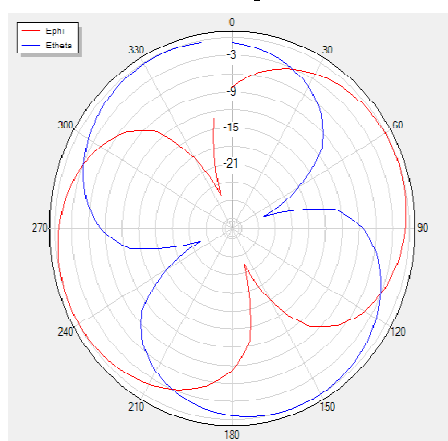
H Theta=0 freq=5400MHz
