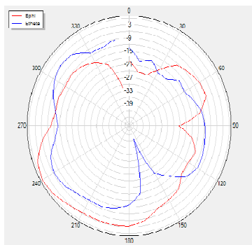
H Theta=90 freq=5100MHz
