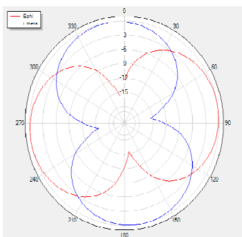
H Theta=0 freq=5100MHz
