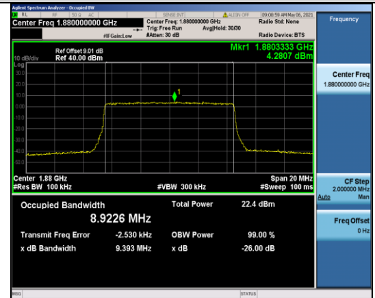
Band2-10MHz-16QAM-18900-50RB#0-8.9226
