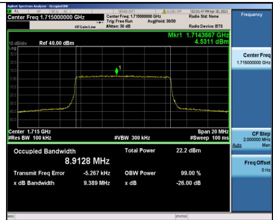
Band4-10MHz-16QAM-20000-50RB#0-8.9128
