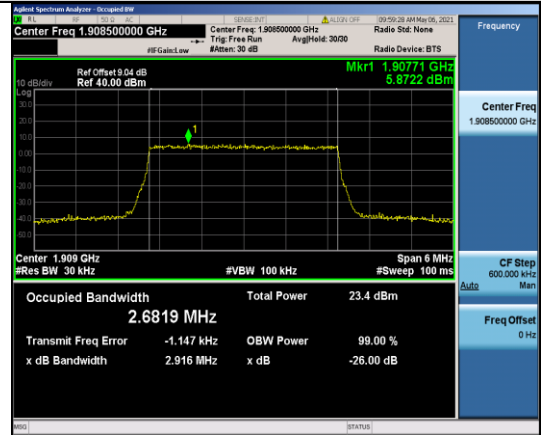
Band2-3MHz-16QAM-19185-15RB#0-2.6819
