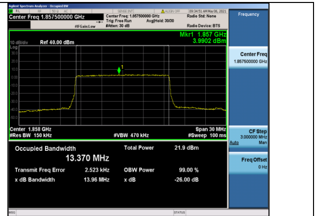
Band2-15MHz-16QAM-18675-75RB#0-13.370
