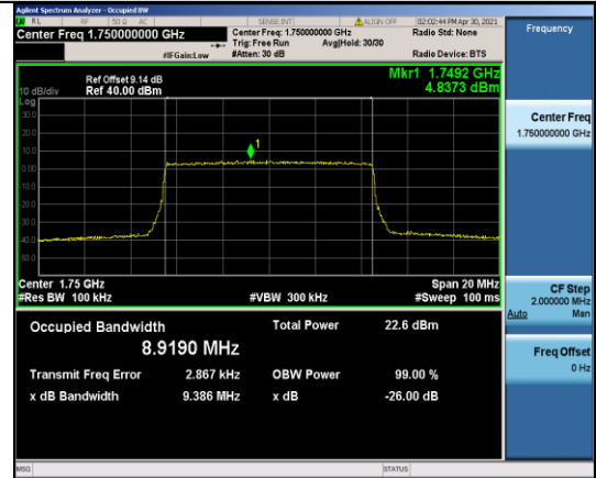
Band4-10MHz-16QAM-20350-50RB#0-8.9190
