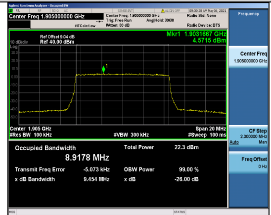
Band2-10MHz-16QAM-19150-50RB#0-8.9178
