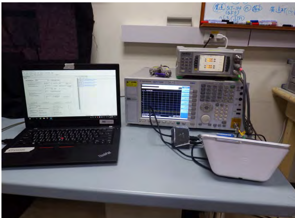
Conducted Setup Photo (Measurement at Antenna Port) (BLE 2M)
