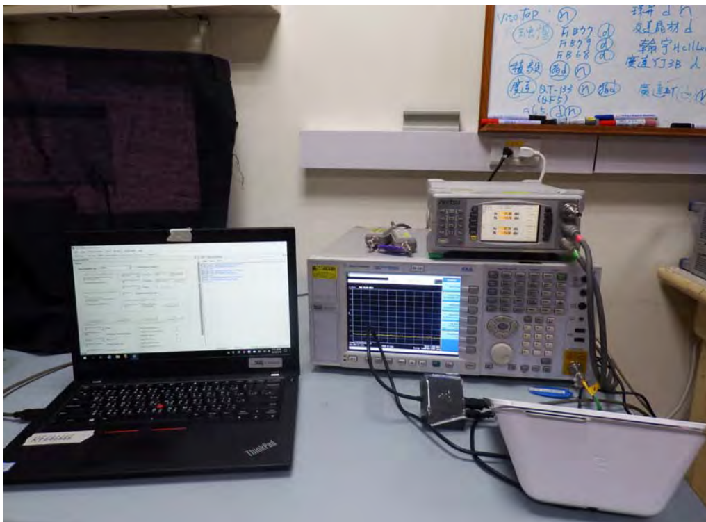
Conducted Setup Photo (Measurement at Antenna Port) (BLE 1M)
