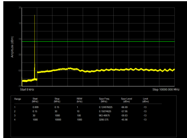
LTE Band 26 10MHz CH-High 9kHz ~10GHz
