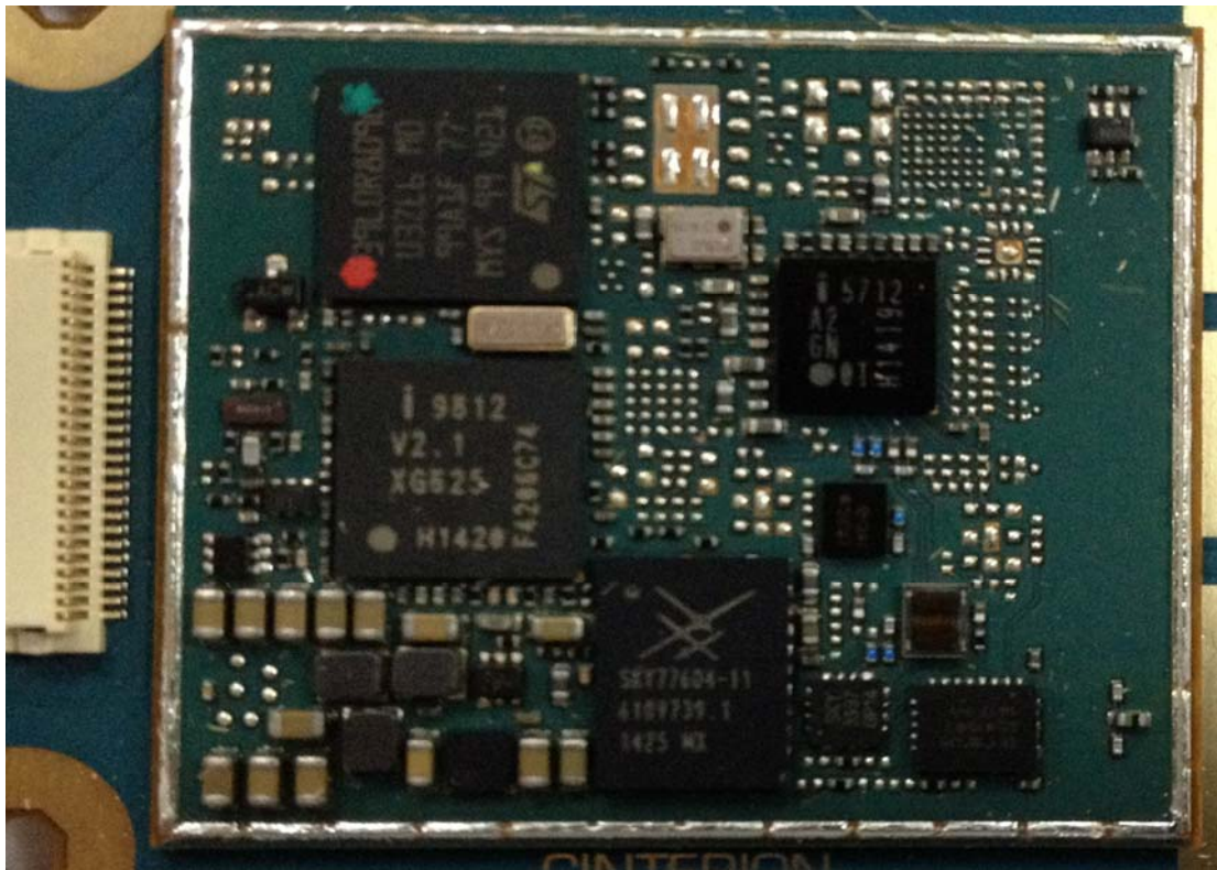
View of EUT-1
