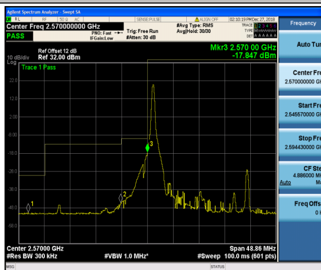
Band38_20MHz_16QAM_37850_1RB#0
