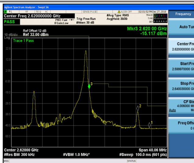
Band38_15MHz_16QAM_38175_1RB#74
