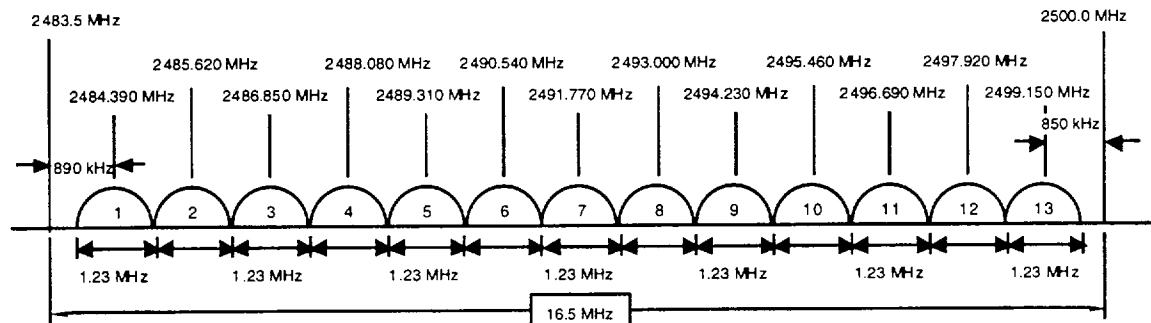
Figure 3-5 S - Band Channel Frequencies
