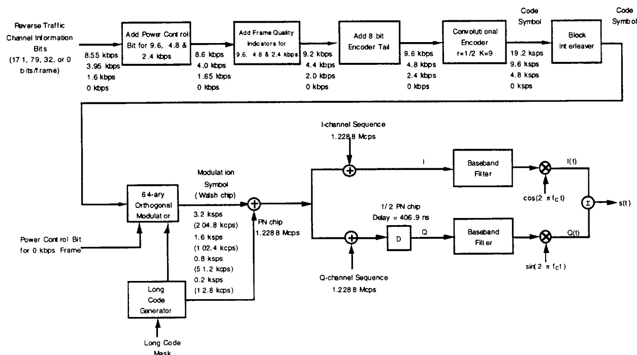
Figure 4-10 Return Link Traffic Channel
