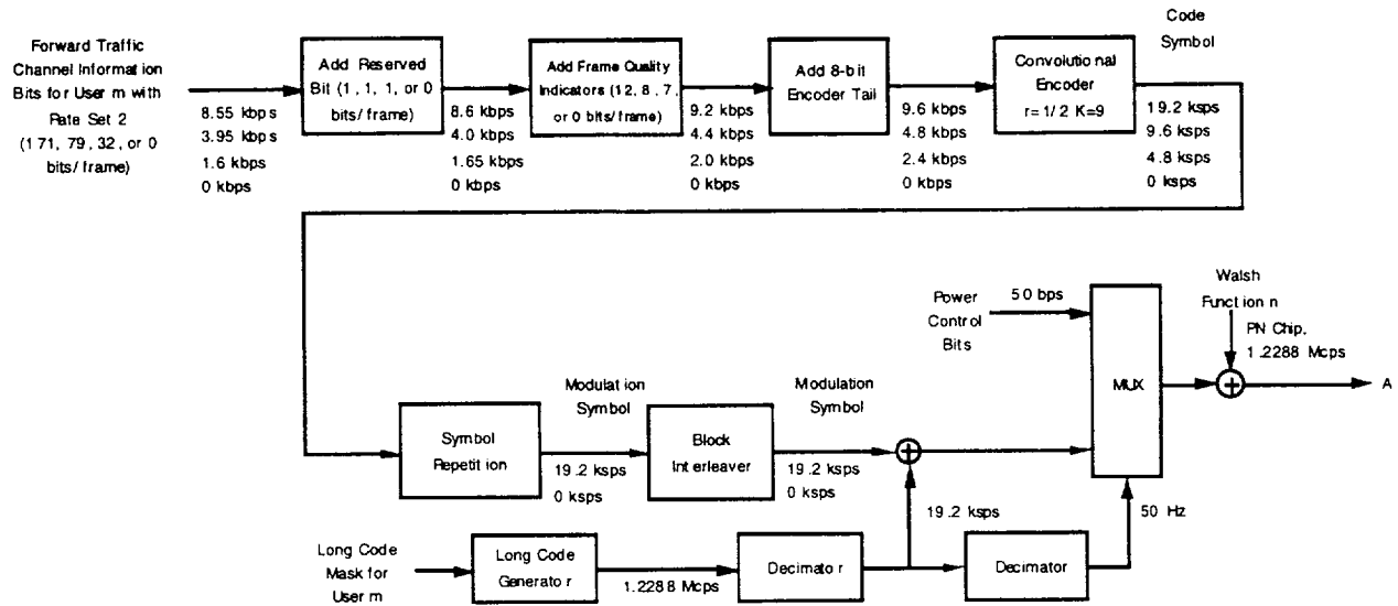
Figure 4-6 Forward Link Traffic Channel - Rate Set 2
