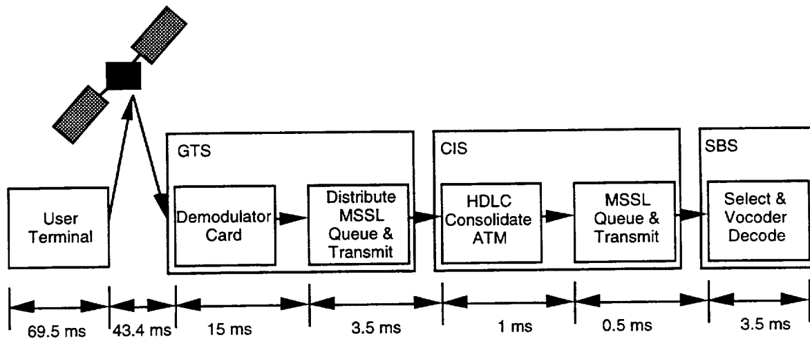
Figure 4-12 Reverse Link Delay Budget
