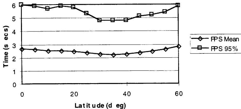
Figure 4-2 Acquisition Time as a function of Latitude
