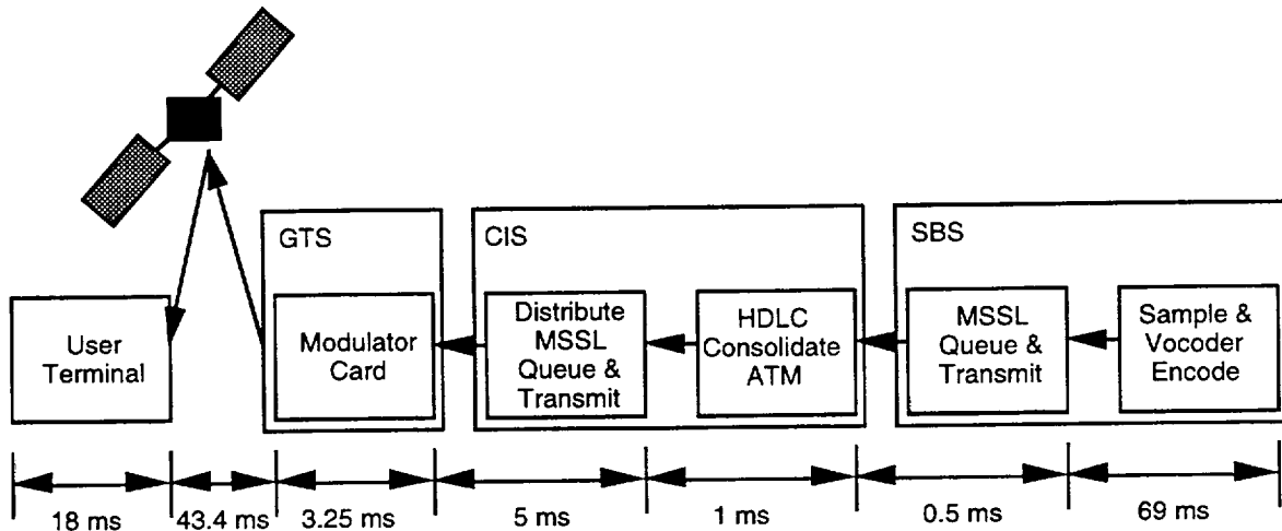
Figure 4-11 Forward Link Delay Budget
