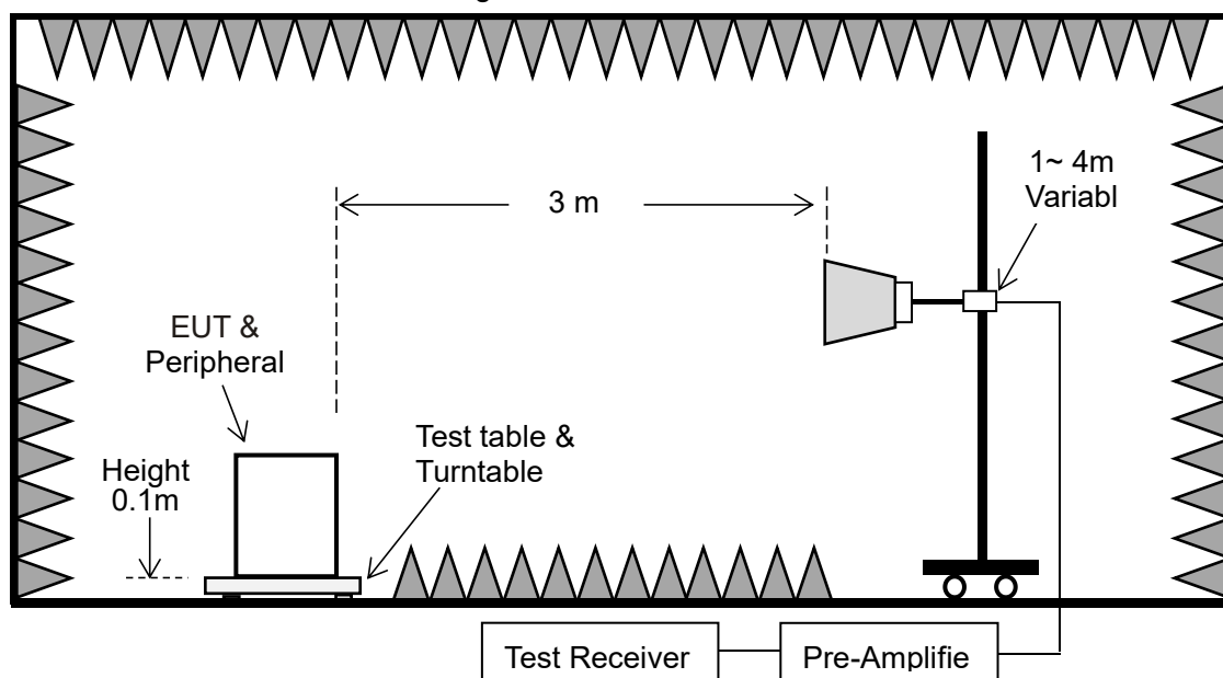
Figure 3. Above 1 GHz
