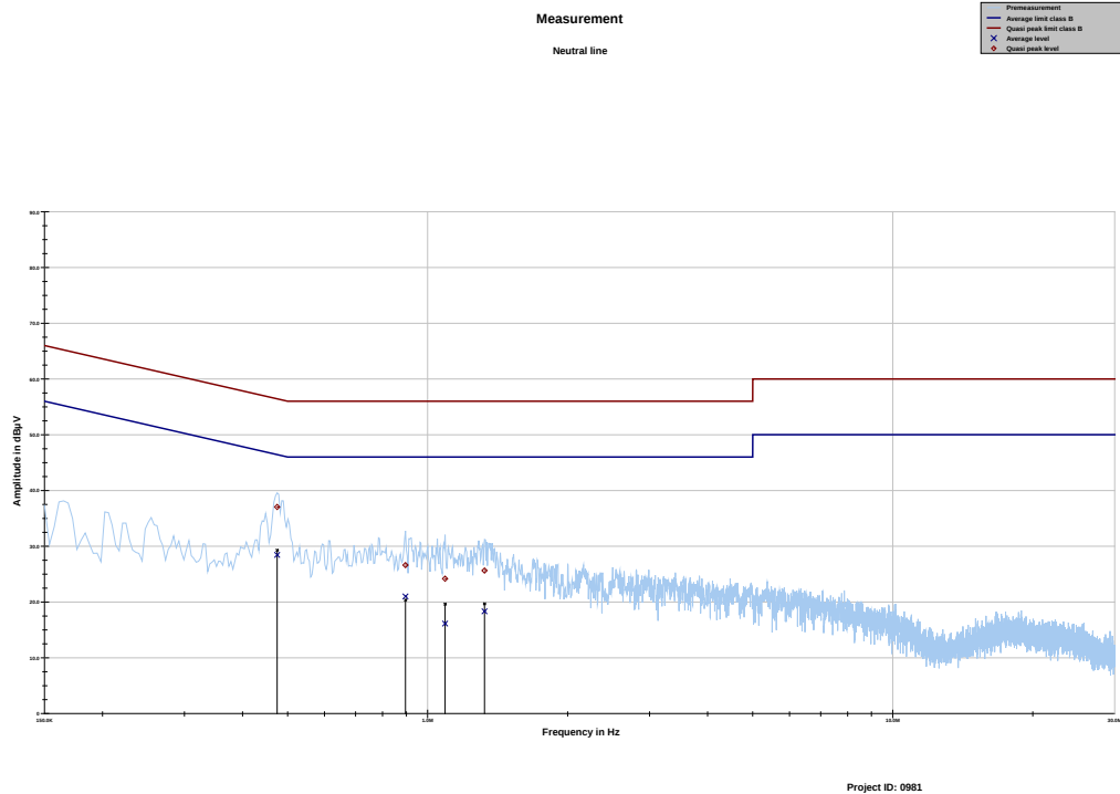
Plot 35: Neutral line
