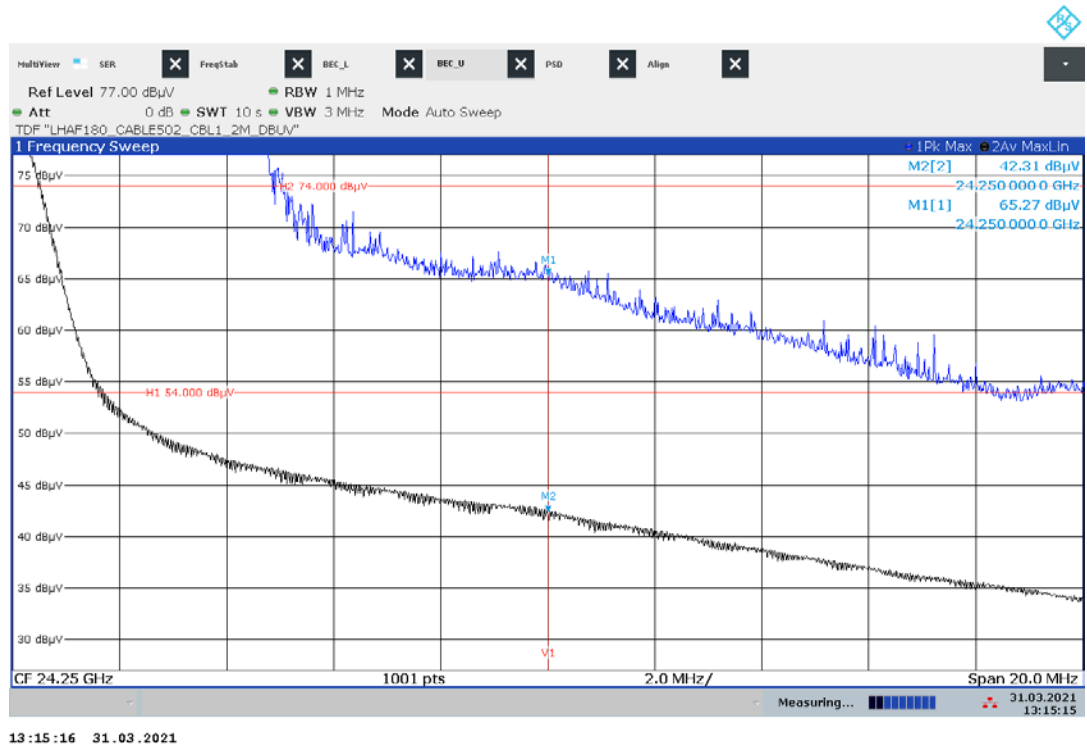
Plot No. 33: Band-Edge-Compliance, high frequency mode, upper edge
