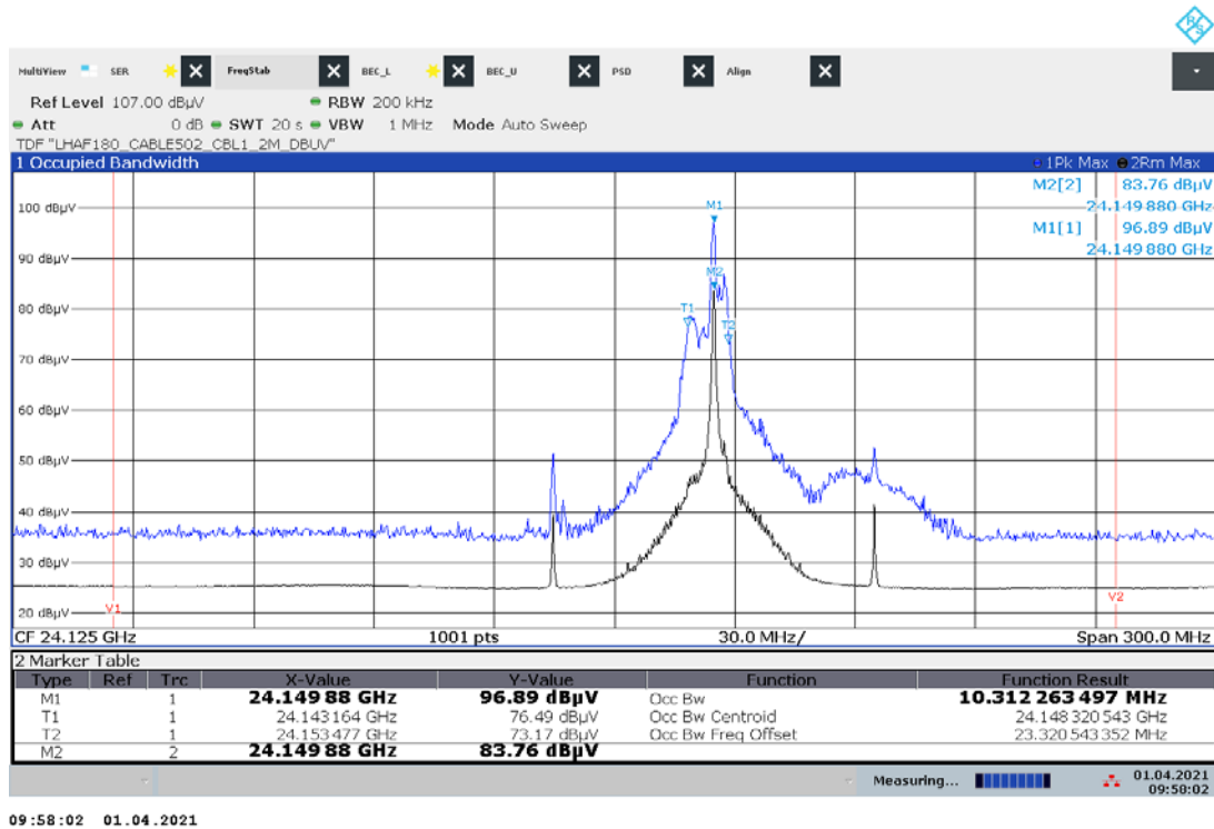
Plot 53: +25 °C, high frequency mode, V_{nom}
