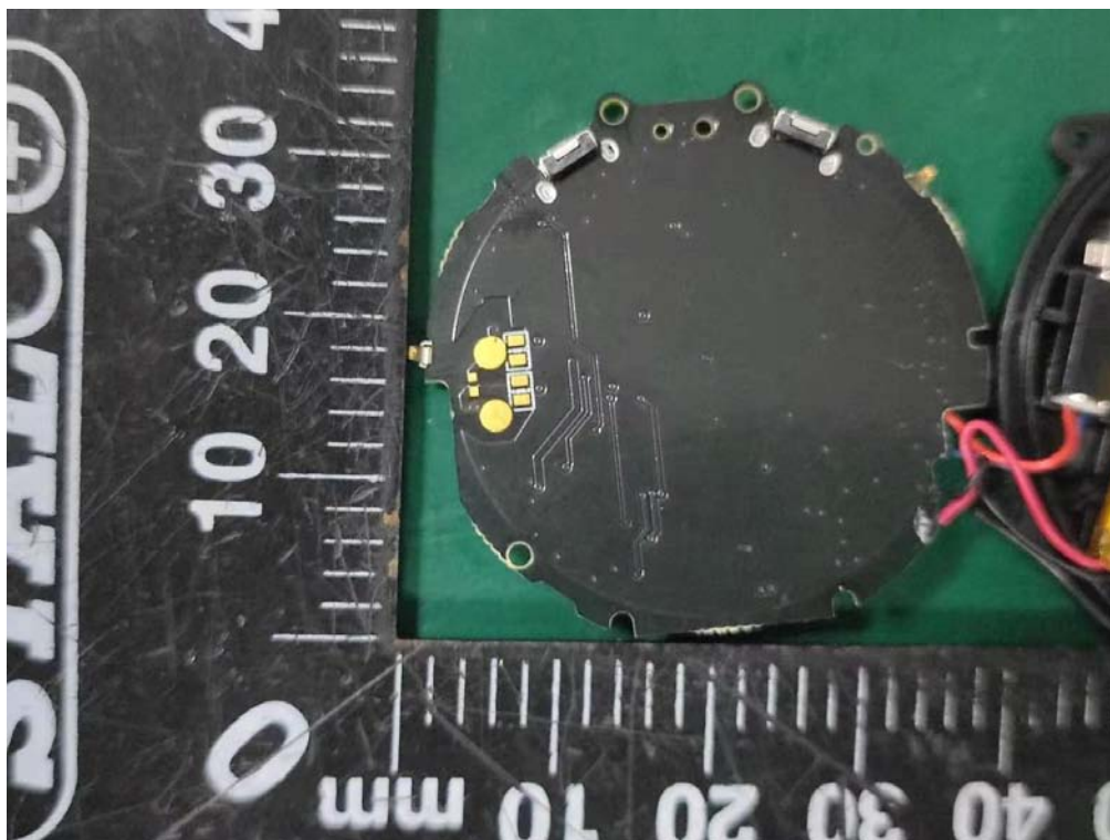
Internal photos M/N: TGW008
