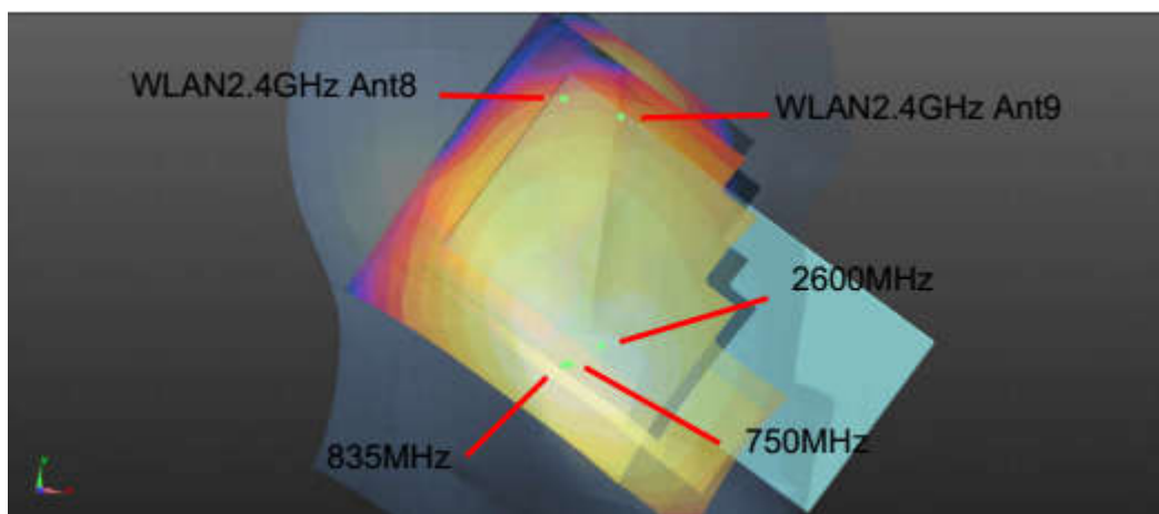
WWAN+WLAN2.4GHz_0mm
