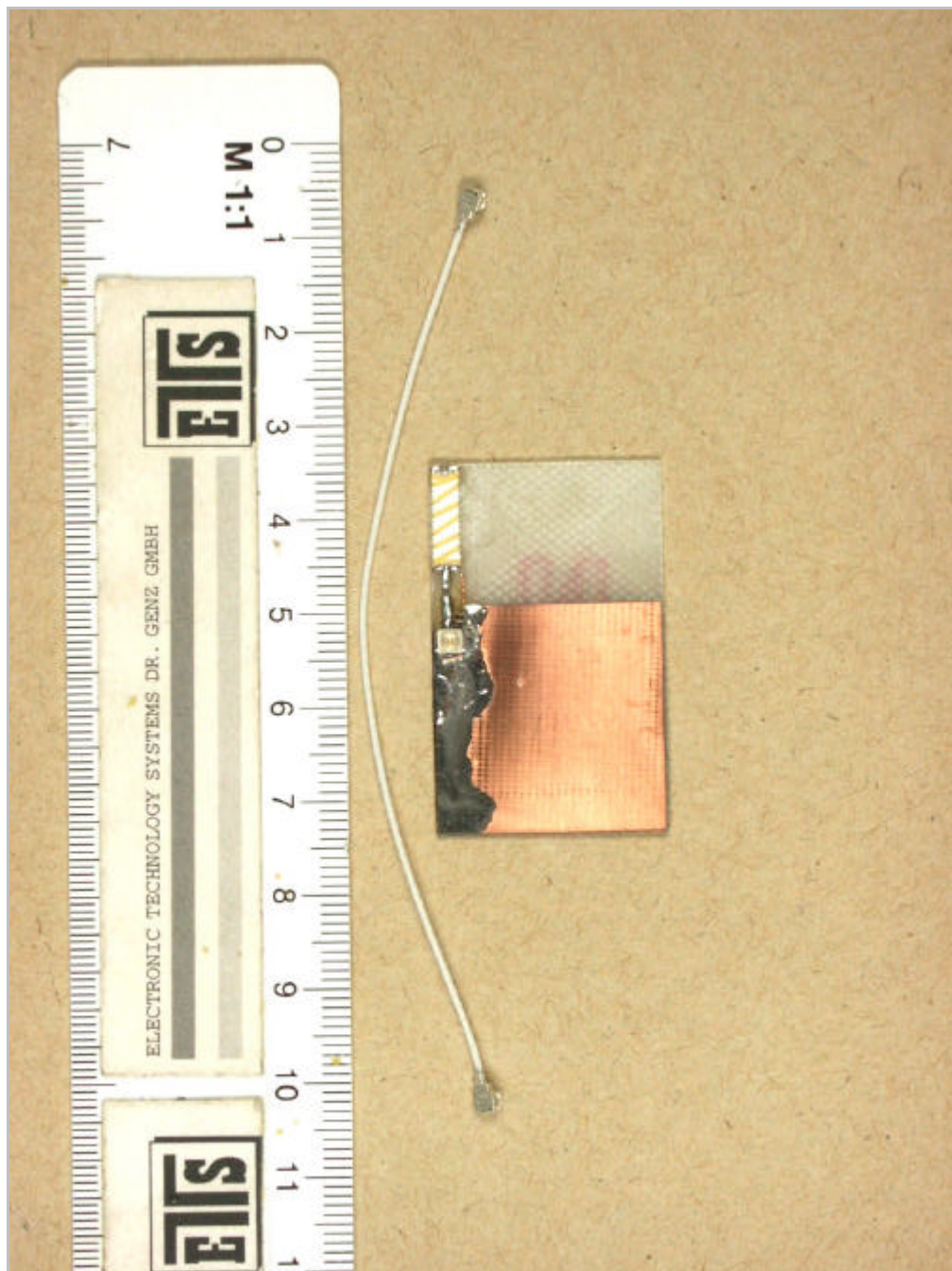
External antenna
