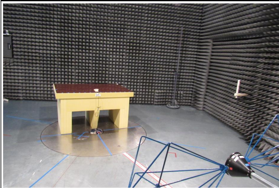
Test setup Operational mode 1
