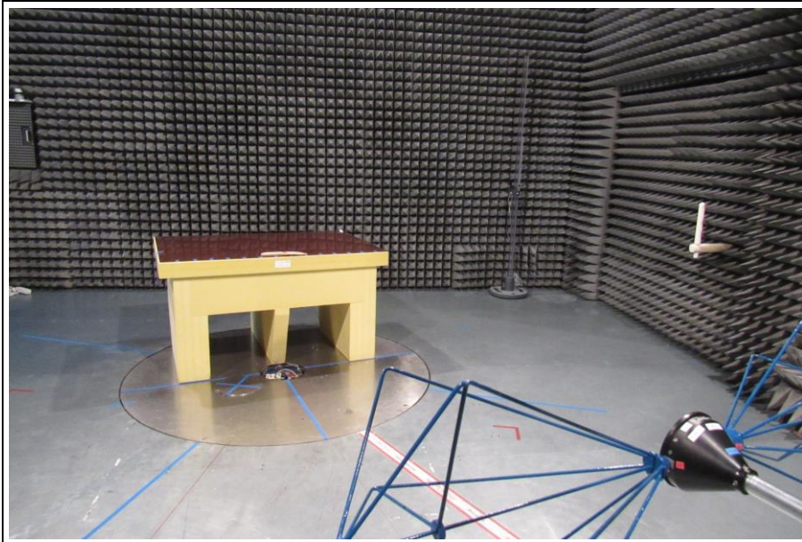
Test setup Operational mode 2
