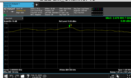
In-Band Reference Level BLE 2M_Channel 39
