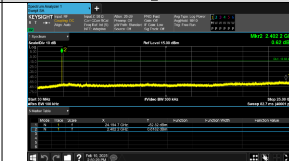
30.0 MHz - 25000.0 MHz BLE 2M_Channel 0
