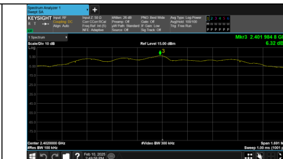
In-Band Reference Level BLE 2M_Channel 0
