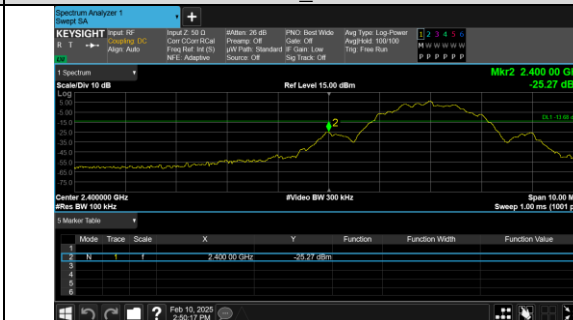
Out Of Band Emission BLE 2M_Channel 0
