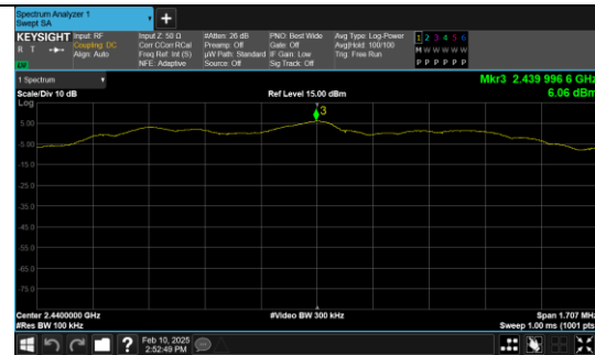
In-Band Reference Level BLE 2M_Channel 19
