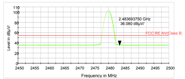
DH5-Channel 78: Average
