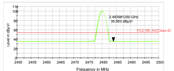
3DH5-Channel 78: Average
