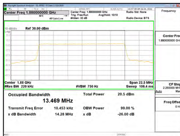
LTE2 15MHz QPSK MID Ch RB15-0
