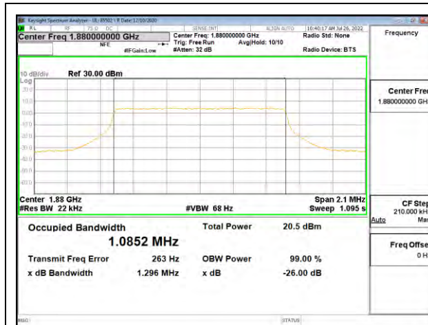
LTE2 1.4MHz QPSK MID Ch RB100-0
