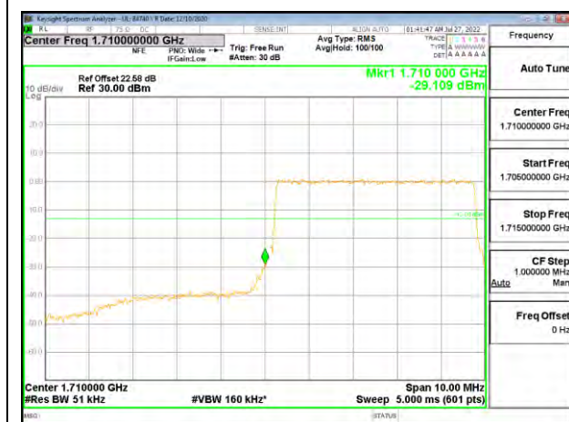
LTE 5MHz 16QAM LOW Ch RB25-0
