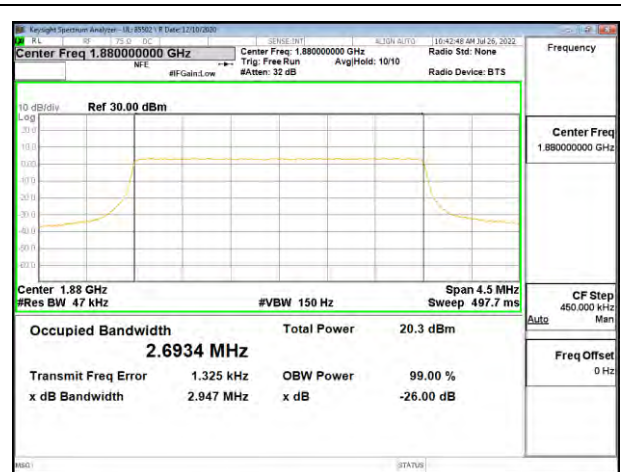
LTE2 3MHz QPSK MID Ch RB75-0
