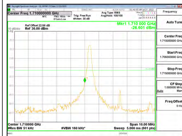
LTE 5MHz 16QAM LOW Ch RB1-0
