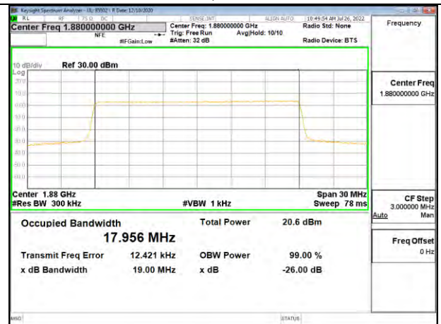
LTE2 20MHz 16QAM MID Ch RB100-0
