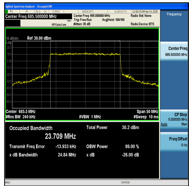
NTNV-n71-PC3-15-25-H-CP-QPSK-Outer_Full-Ant1-PASS
