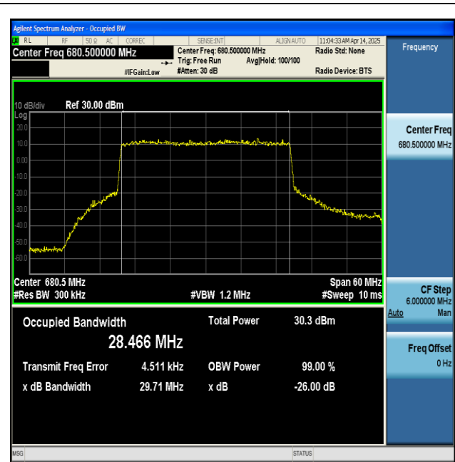
NTNV-n71-PC3-15-30-M-CP-QPSK-Outer_Full-Ant1-PASS
