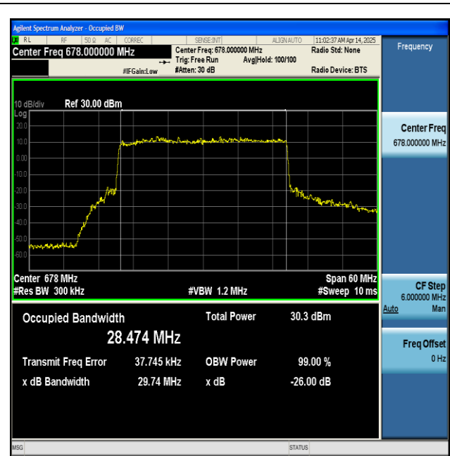
NTNV-n71-PC3-15-30-L-CP-16QAM-Outer_Full-Ant1-PASS
