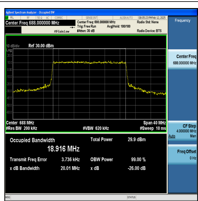
NTNV-n71-PC3-15-20-H-CP-16QAM-Outer_Full-Ant1-PASS
