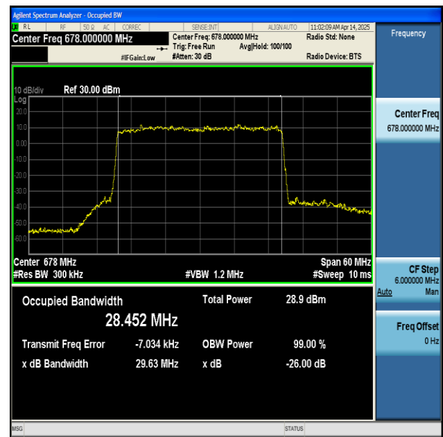
NTNV-n71-PC3-15-30-L-DFT-256QAM-Outter_Full-Ant1-PASS
