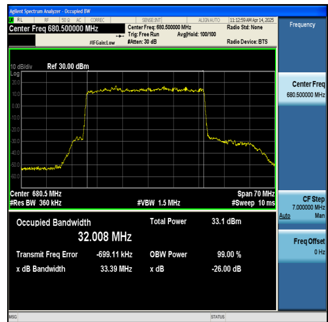
NTNV-n71-PC3-15-35-M-DFT-BPSK-Outer_Full-Ant1-PASS
