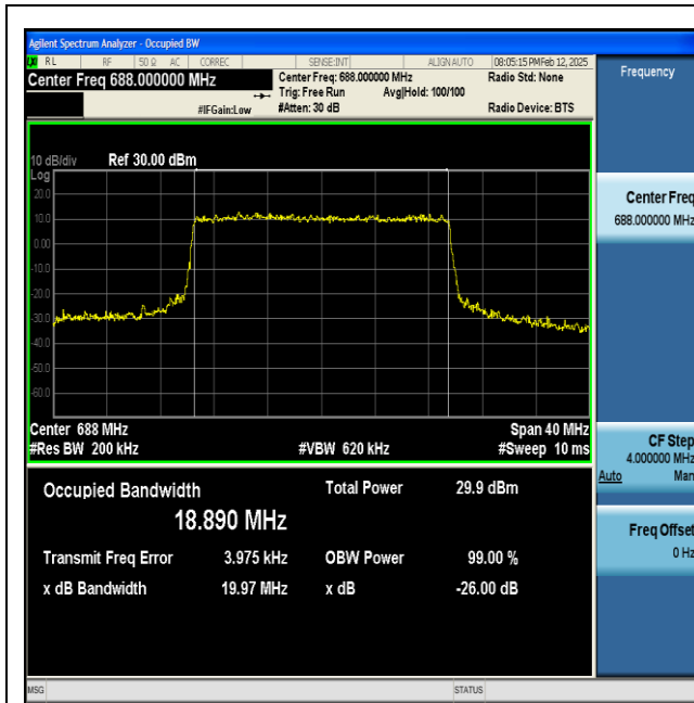
NTNV-n71-PC3-15-20-H-CP-QPSK-Outer_Full-Ant1-PASS
