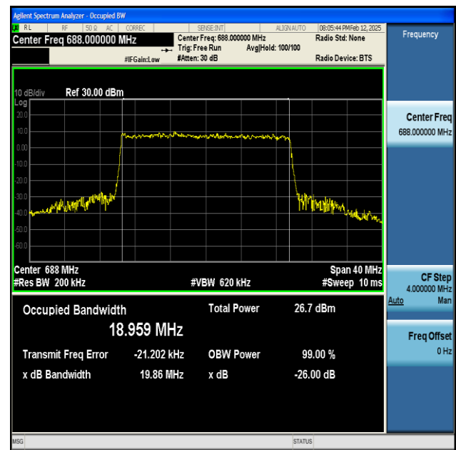
NTNV-n71-PC3-15-20-H-CP-256QAM-Outer_Full-Ant1-PASS
