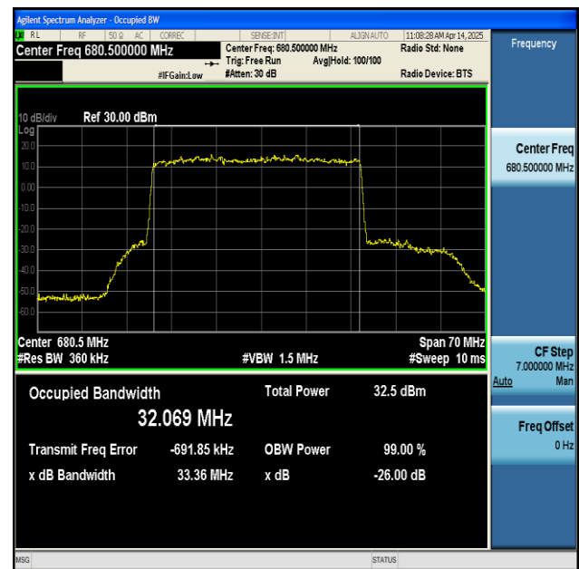
NTNV-n71-PC3-15-35-L-CP-QPSK-Outer_Full-Ant1-PASS
