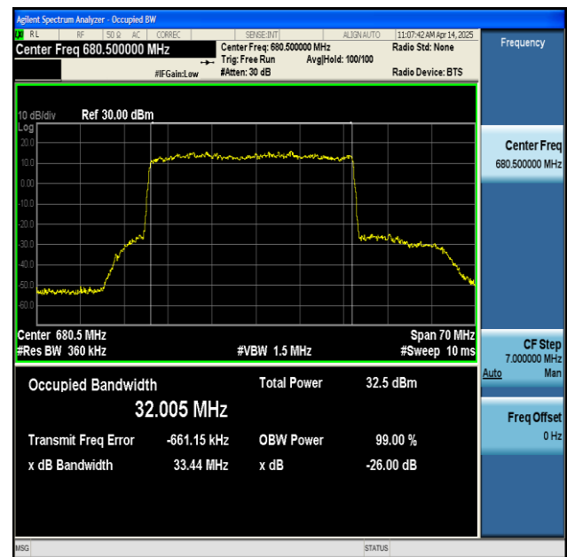
NTNV-n71-PC3-15-35-L-DFT-QPSK-Outer_Full-Ant1-PASS
