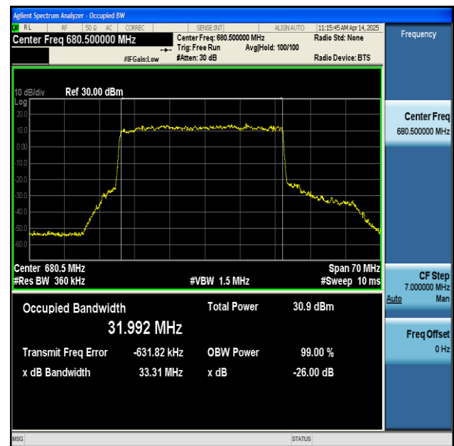
NTNV-n71-PC3-15-35-H-DFT-64QAM-Outer_Full-Ant1-PASS
