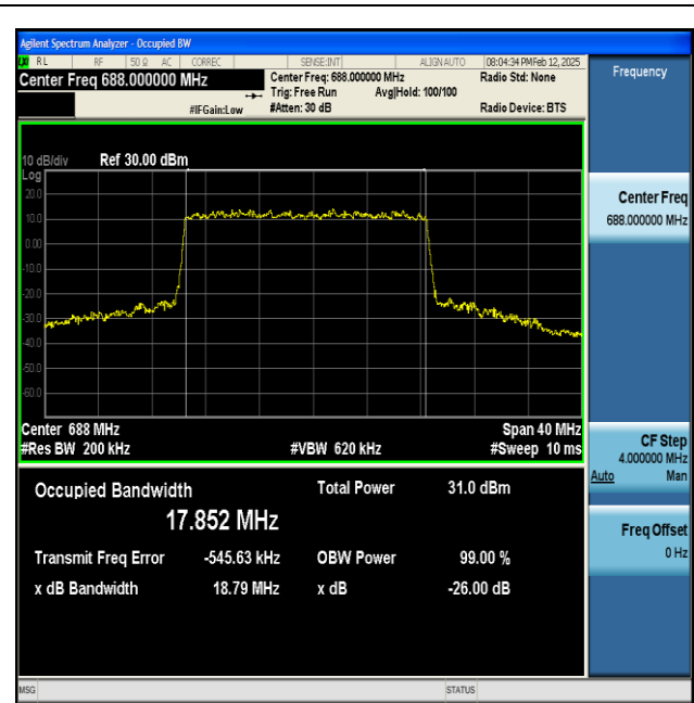
NTNV-n71-PC3-15-20-H-DFT-16QAM-Outter_Full-Ant1-PASS
