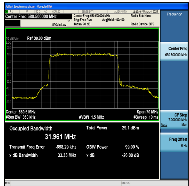
NTNV-n71-PC3-15-35-M-DFT-256QAM-Outet_Full-Ant1-PASS
