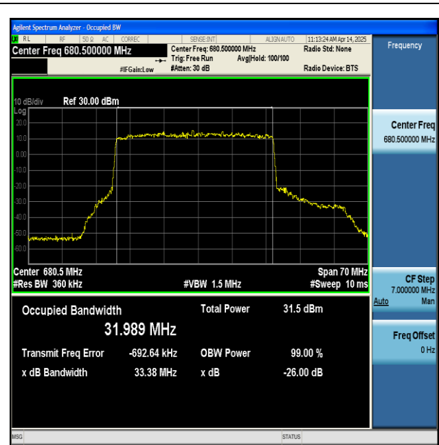
NTNV-n71-PC3-15-35-M-DFT-16QAM-Outet_Full-Ant1-PASS
