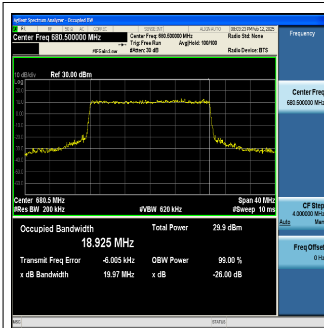
NTNV-n71-PC3-15-20-M-CP-16QAM-Outer_Full-Ant1-PASS
