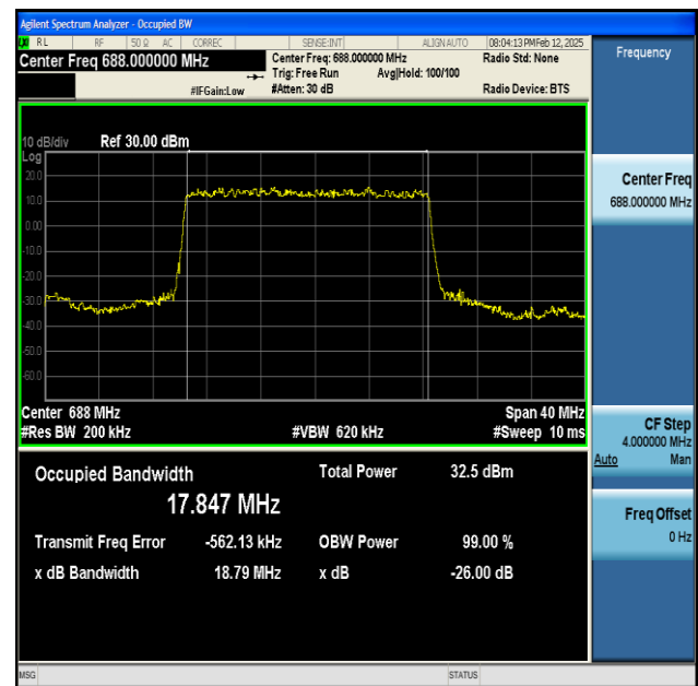
NTNV-n71-PC3-15-20-H-DFT-BPSK-Outer_Full-Ant1-PASS
