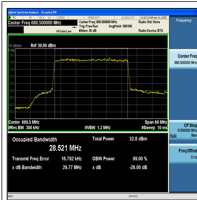
NTNV-n71-PC3-15-30-M-DFT-BPSK-Outter_Full-Ant1-PASS
