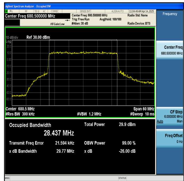
NTNV-n71-PC3-15-30-M-CP-64QAM-Outer_Full-Ant1-PASS
