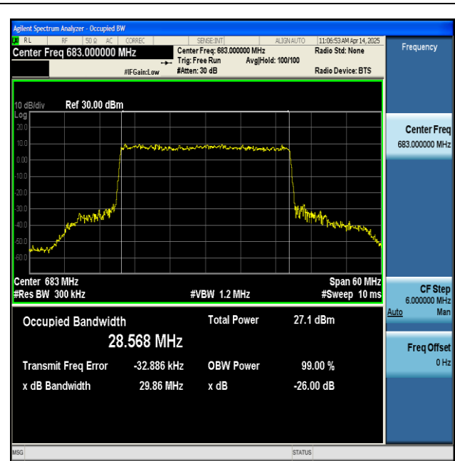
NTNV-n71-PC3-15-30-H-CP-256QAM-Outer_Full-Ant1-PASS
