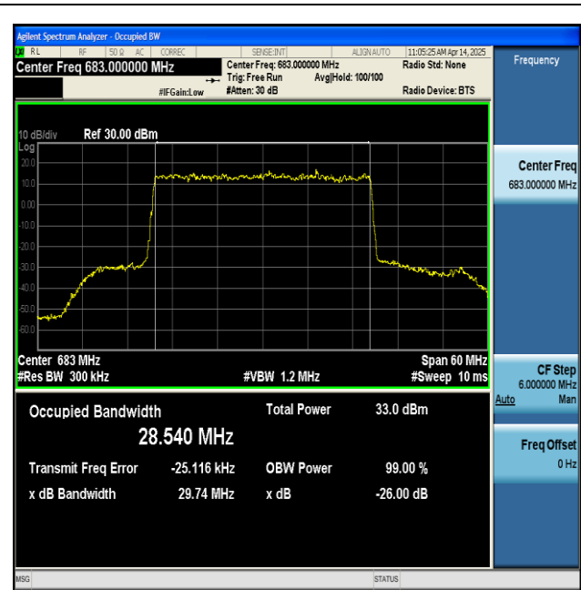
NTNV-n71-PC3-15-30-H-DFT-BPSK-Outer_Full-Ant1-PASS
