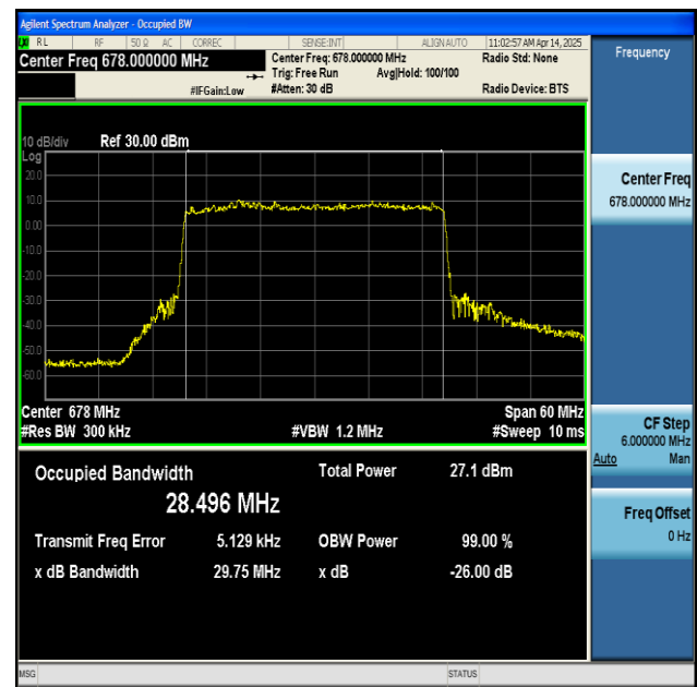
NTNV-n71-PC3-15-30-L-CP-256QAM-Outer_Full-Ant1-PASS
