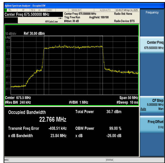
NTNV-n71-PC3-15-25-L-DFT-64QAM-Outer_Full-Ant1-PASS
