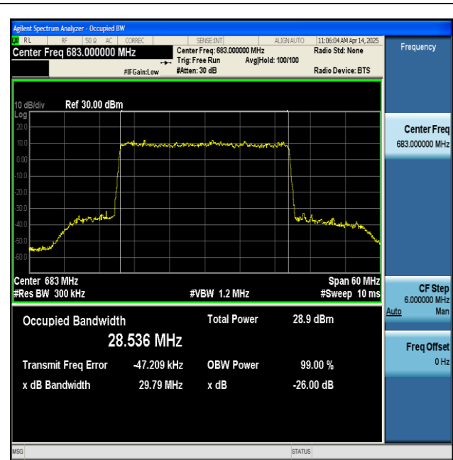
NTVN-n71-PC3-15-30-H-DFT-256QAM-Outer_Full-Ant1-PASS
