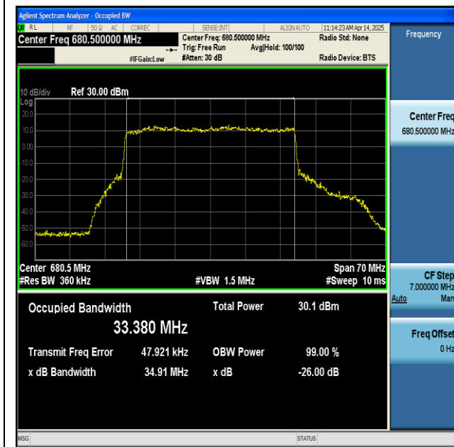
NTNV-n71-PC3-15-35-M-CP-64QAM-Outer_Full-Ant1-PASS
