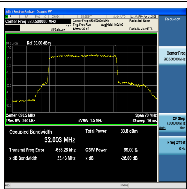
NTNV-n71-PC3-15-35-H-DFT-QPSK-Outer_Full-Ant1-PASS
