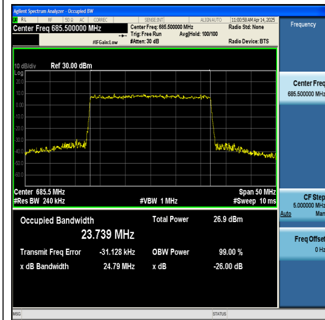
NTNV-n71-PC3-15-25-H-CP-256QAM-Outer_Full-Ant1-PASS
