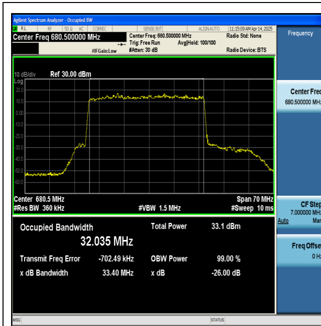
NTNV-n71-PC3-15-35-H-DFT-BPSK-Outer_Full-Ant1-PASS
