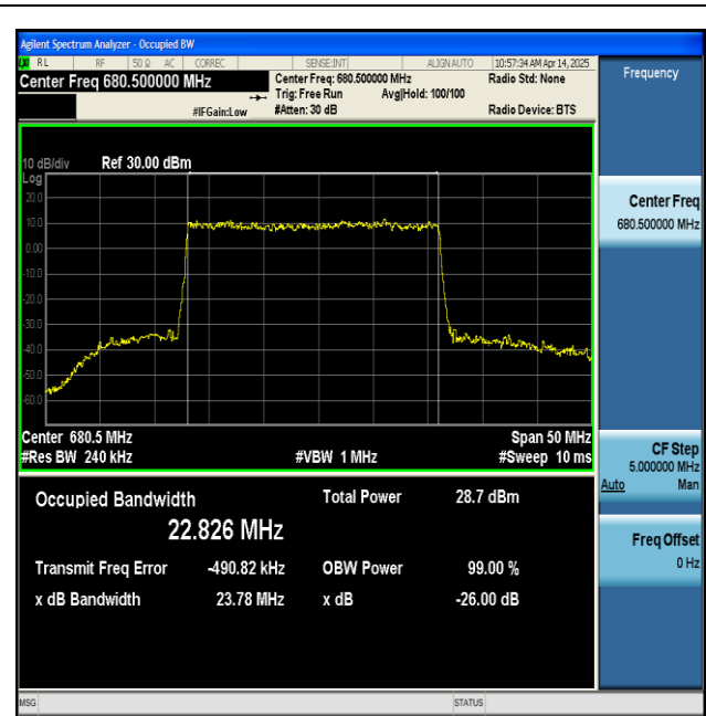
NTNV-n71-PC3-15-25-M-DFT-256QAM-Outer_Full-Ant1-PASS
