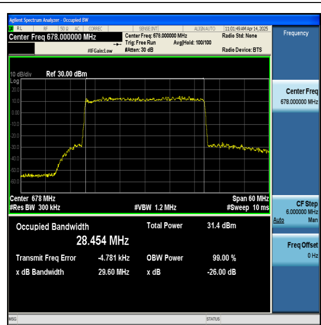
NTNV-n71-PC3-15-30-L-DFT-16QAM-Outter_Full-Ant1-PASS
