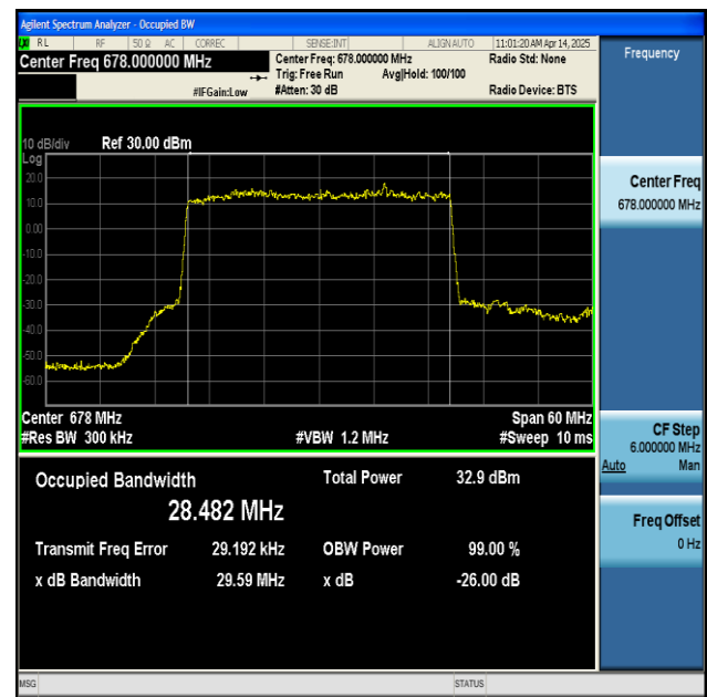
NTNV-n71-PC3-15-30-L-DFT-BPSK-Outer_Full-Ant1-PASS
