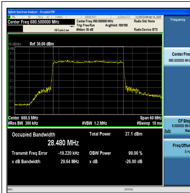
NTNV-n71-PC3-15-30-M-CP-256QAM-Outer_Full-Ant1-PASS
