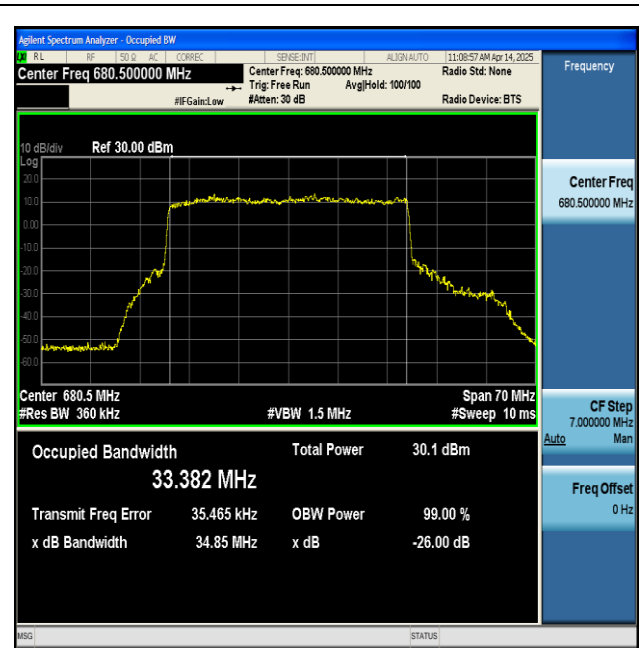
NTNV-n71-PC3-15-35-L-CP-64QAM-Outer_Full-Ant1-PASS
