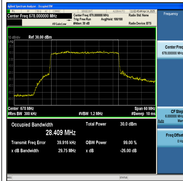
NTNV-n71-PC3-15-30-L-CP-64QAM-Outer_Full-Ant1-PASS
