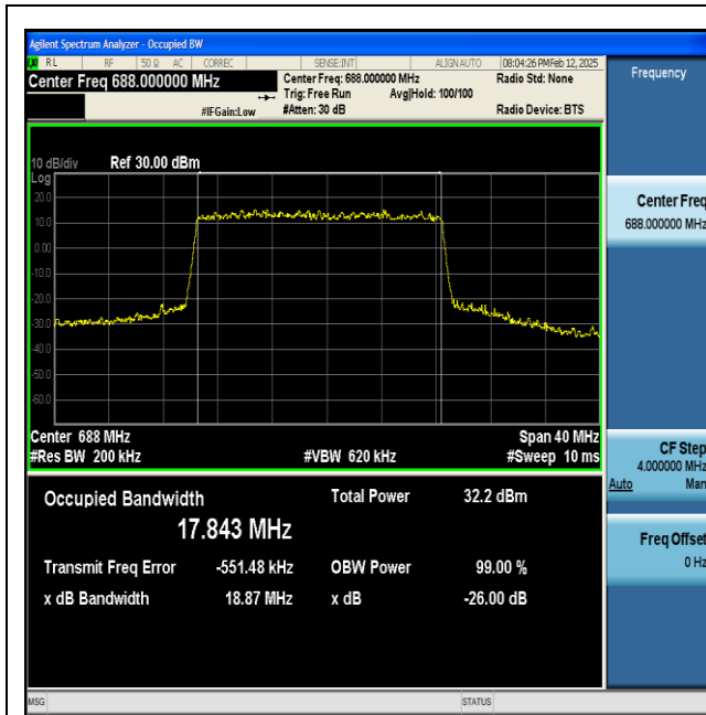
NTNV-n71-PC3-15-20-H-DFT-QPSK-Outter_Full-Ant1-PASS
