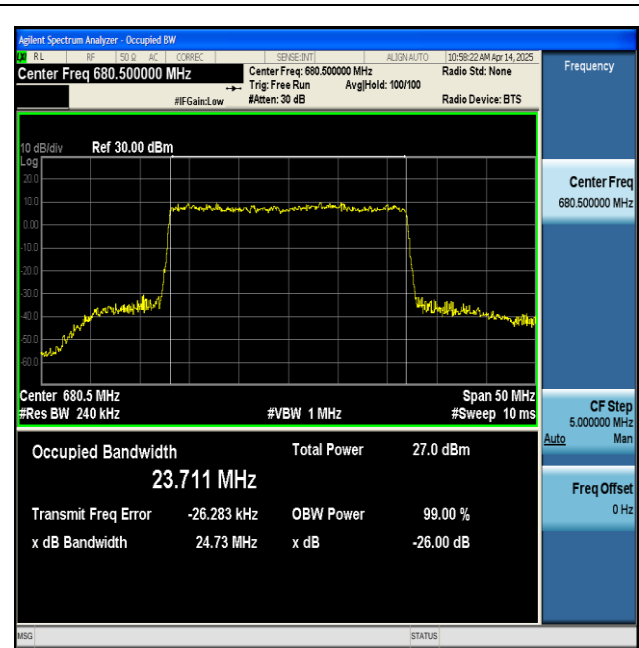
NTNV-n71-PC3-15-25-M-CP-256QAM-Outer_Full-Ant1-PASS
