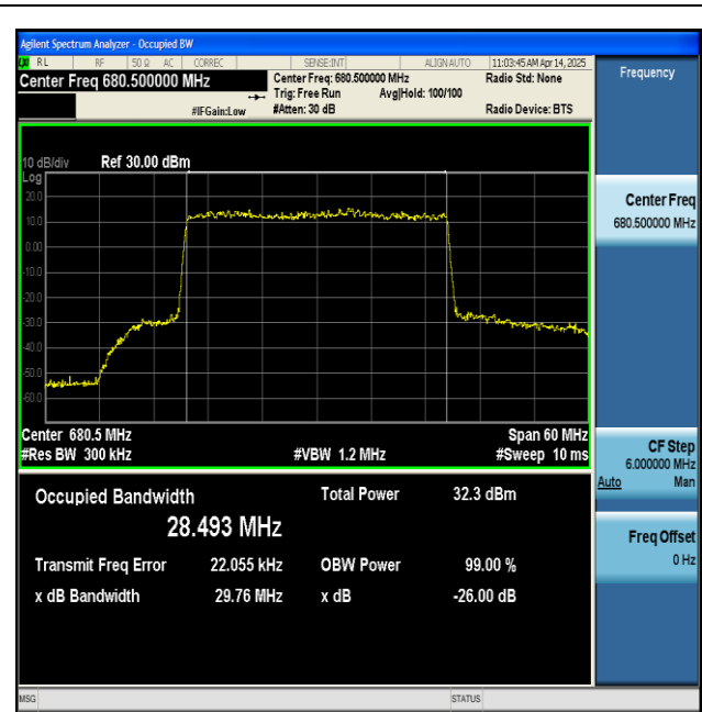
NTNV-n71-PC3-15-30-M-DFT-QPSK-Outter_Full-Ant1-PASS
