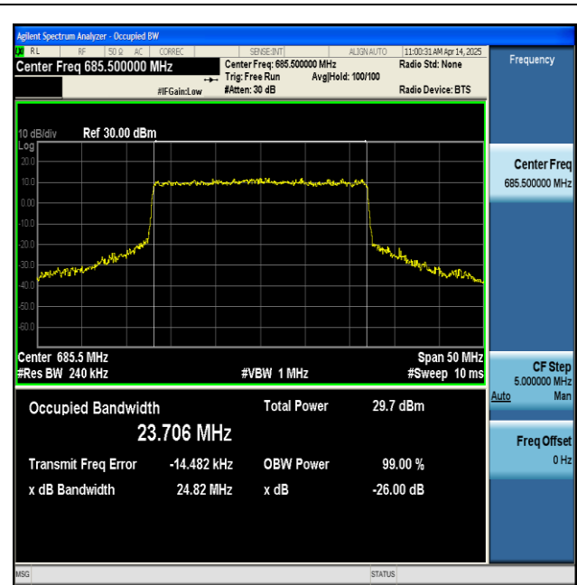
NTNV-n71-PC3-15-25-H-CP-64QAM-Outer_Full-Ant1-PASS
