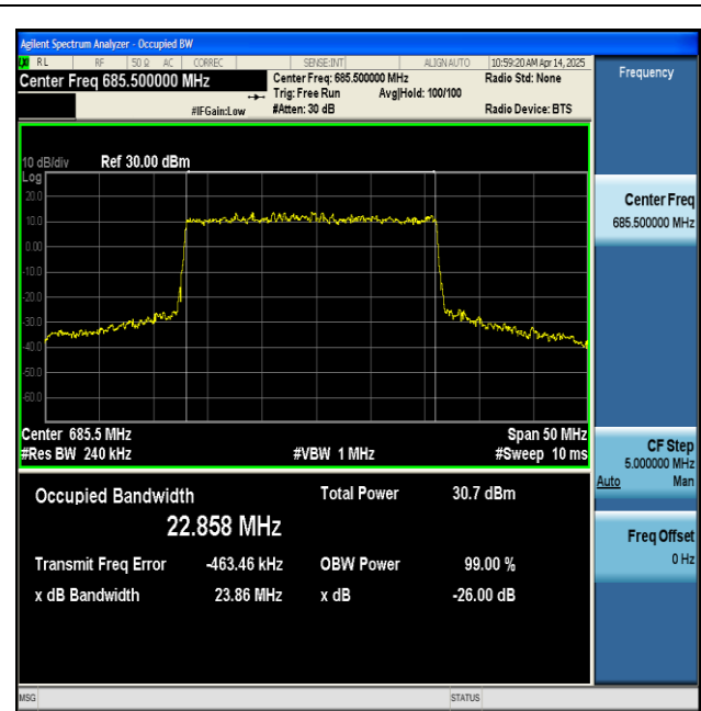
NTNV-n71-PC3-15-25-H-DFT-64QAM-Outer_Full-Ant1-PASS
