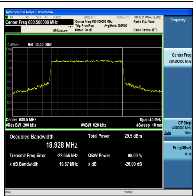
NTNV-n71-PC3-15-20-M-CP-64QAM-Outer_Full-Ant1-PASS
