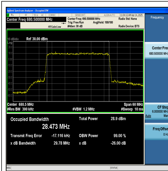
NTNV-n71-PC3-15-30-M-DFT-256QAM-Outer_Full-Ant1-PASS
