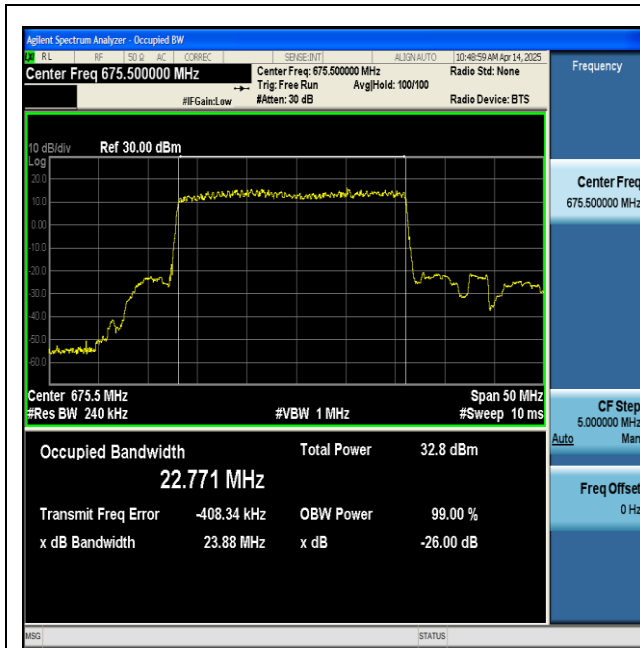
NTNV-n71-PC3-15-25-L-DFT-BPSK-Outer_Full-Ant1-PASS
