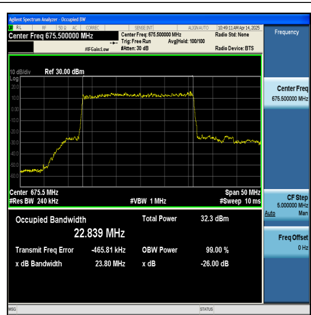
NTNV-n71-PC3-15-25-L-DFT-QPSK-Outer_Full-Ant1-PASS
