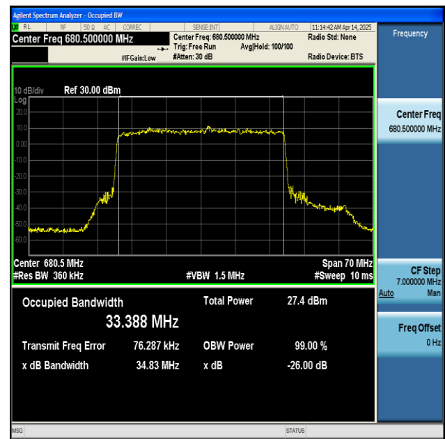
NTNV-n71-PC3-15-35-M-CP-256QAM-Outer_Full-Ant1-PASS
