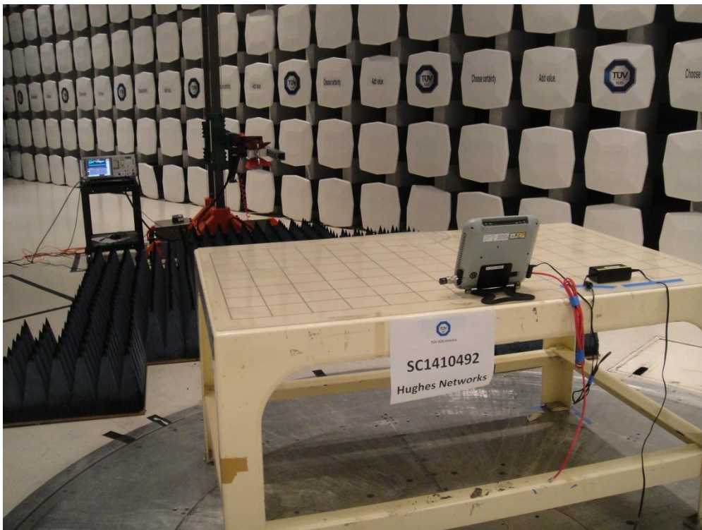
FCC – Radiated Emission Above 1GHz Front and Back
