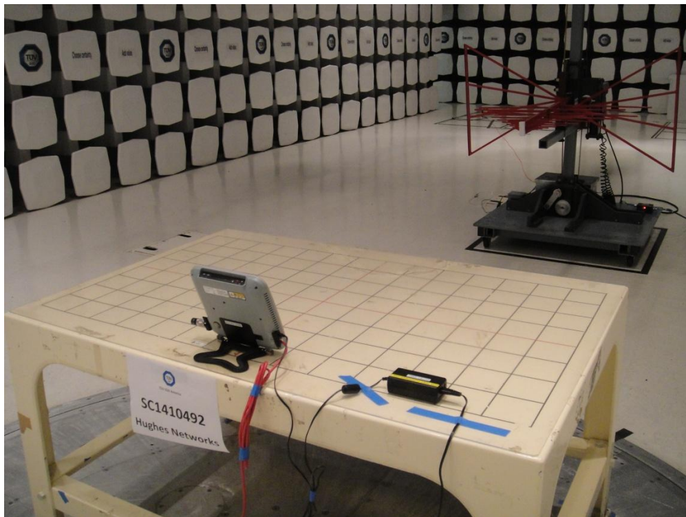
FCC – Radiated Emission Below 1GHz Front and Back
