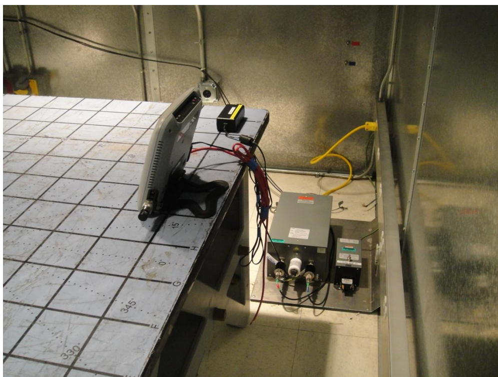
Conducted Emission Front and Back
