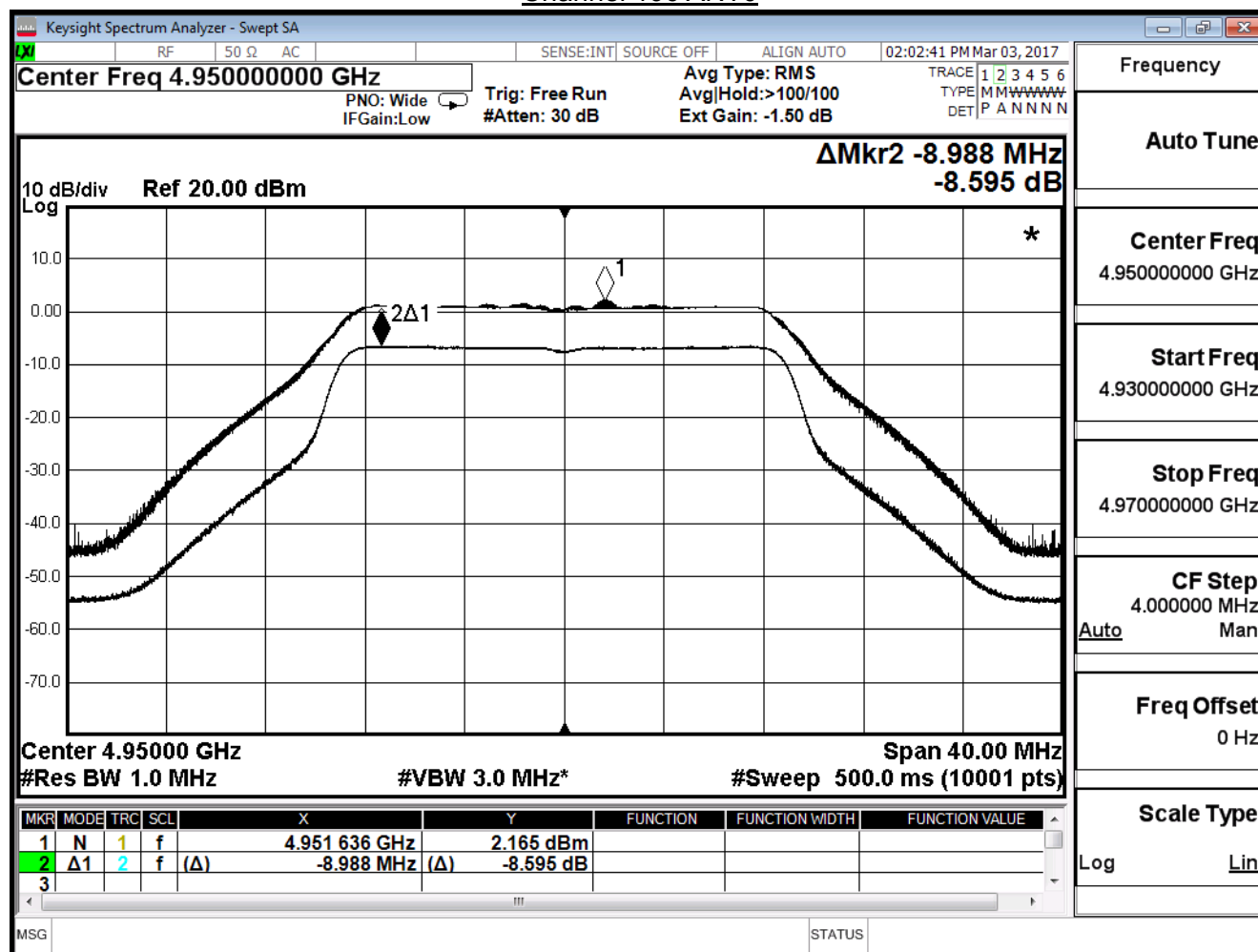
Channel 190 ANT0
