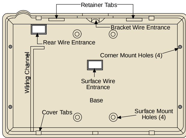
Figure 2: DS720i Base
