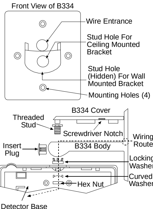
Figure 7: Mounting the B334 Bracket
