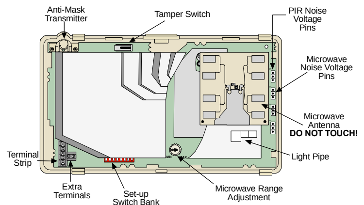
Figure 1: Inside View of DS720i
