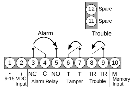
Figure 6: Wiring the DS720i Terminals
