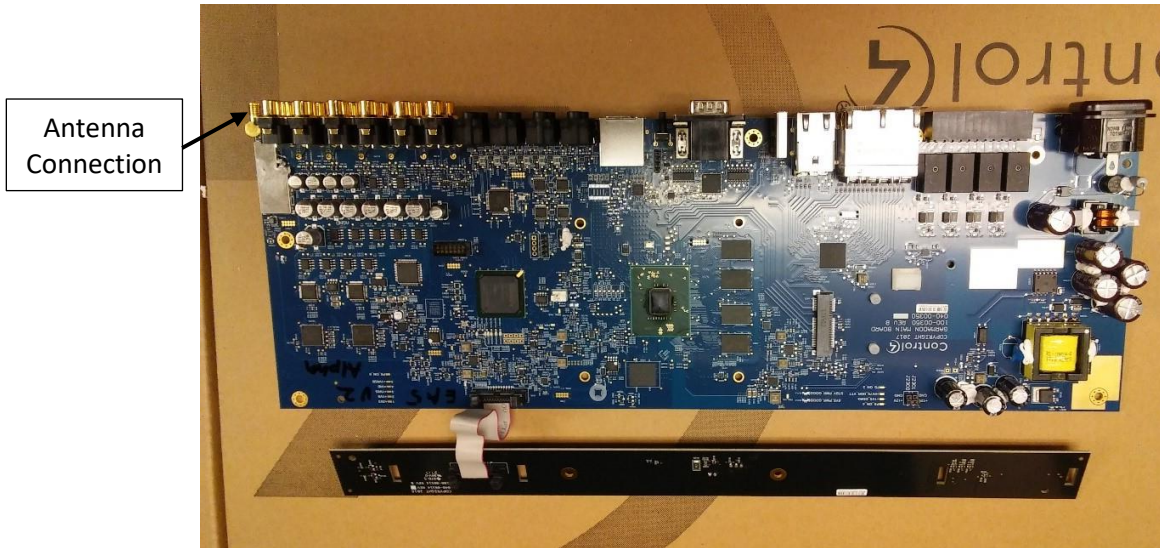
Photograph 1 – Top View of the PCB with Shield
