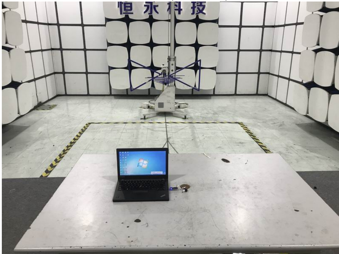
Radiated Test (Below 1GHz)
